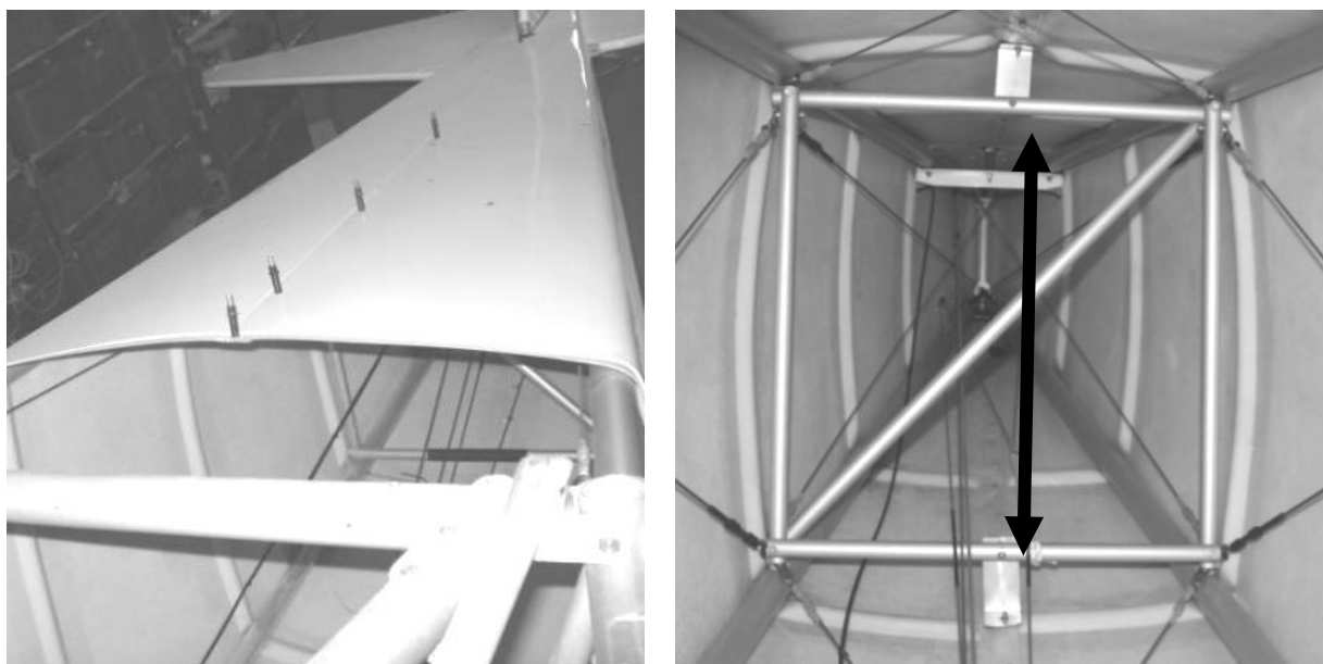
Figure 122 fuselage fairing seams held together with Cleco's, bracing angles
