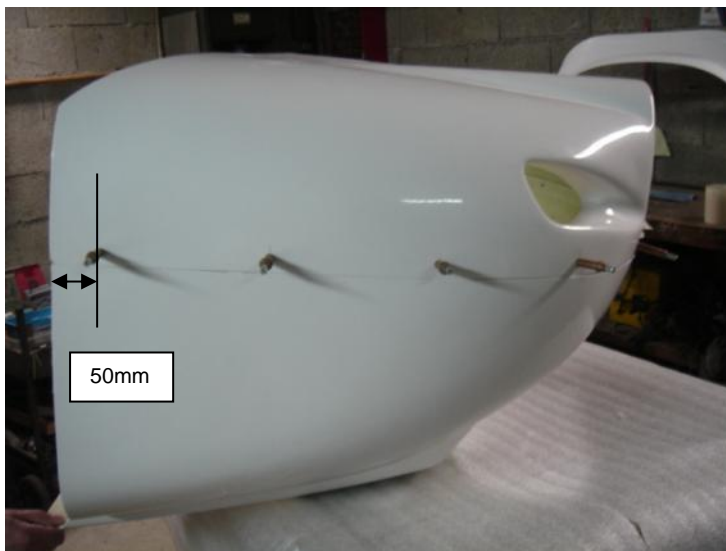
Figure 190 position and spacing of fixings on side of cowling
