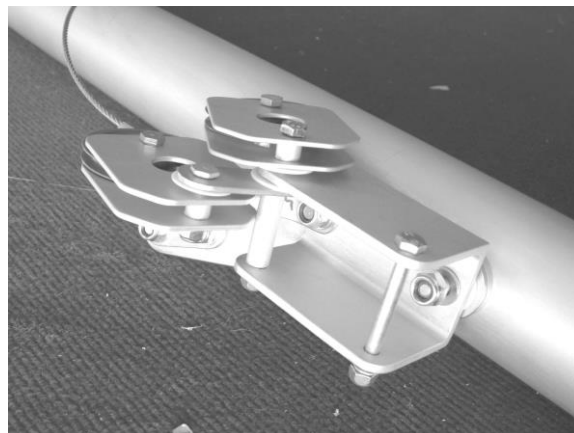
Figure 138 UKMOD aileron pulleys.
