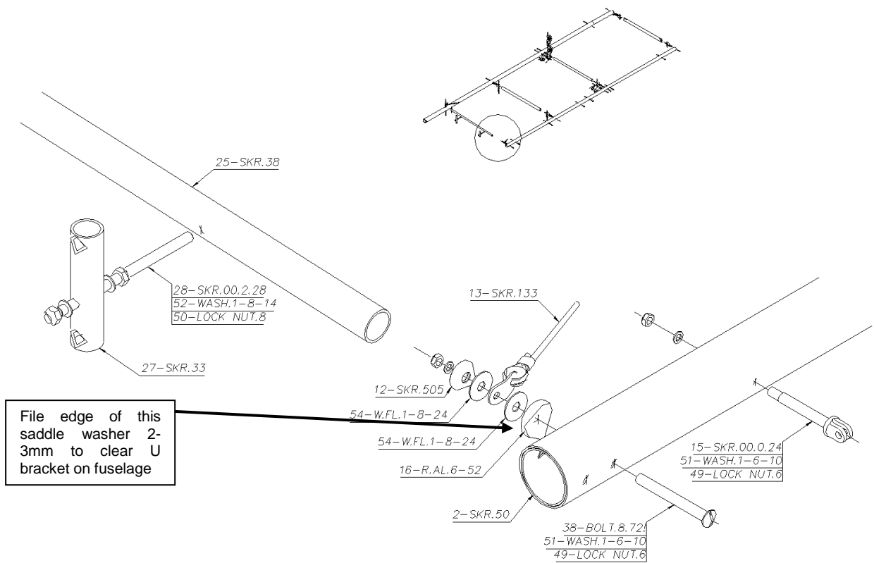
Figure 141 front and rear of tensioning tube.
