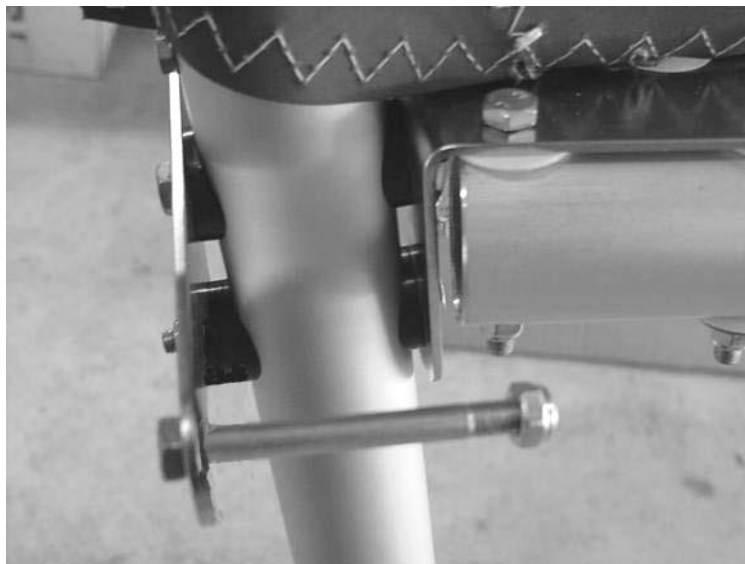
Figure 57 vertical fin and horizontal stabiliser rear mountings.
