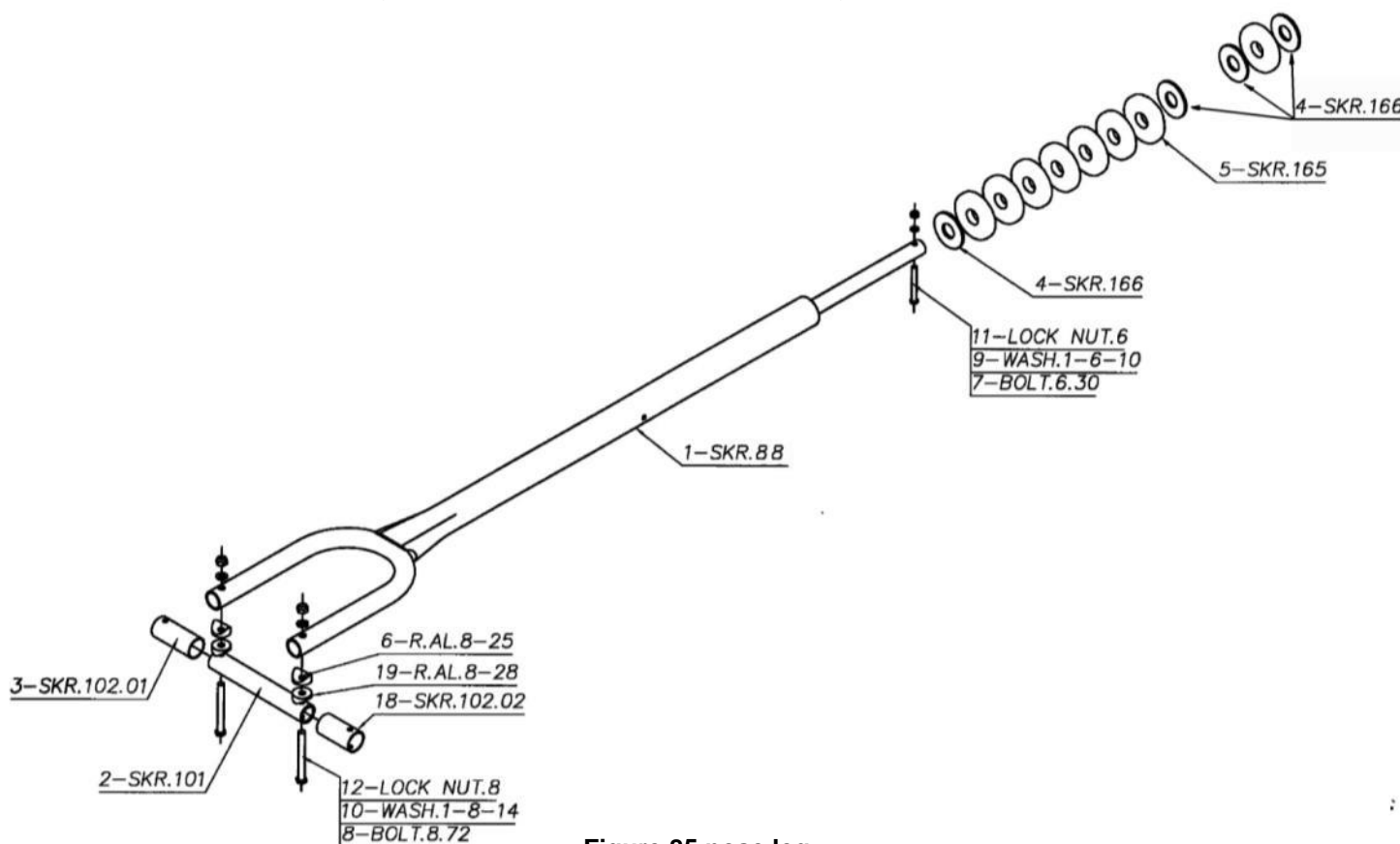
Figure 85 nose leg
