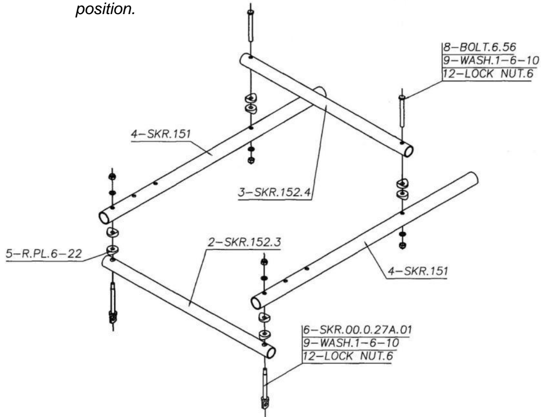
Figure 331 seat base
