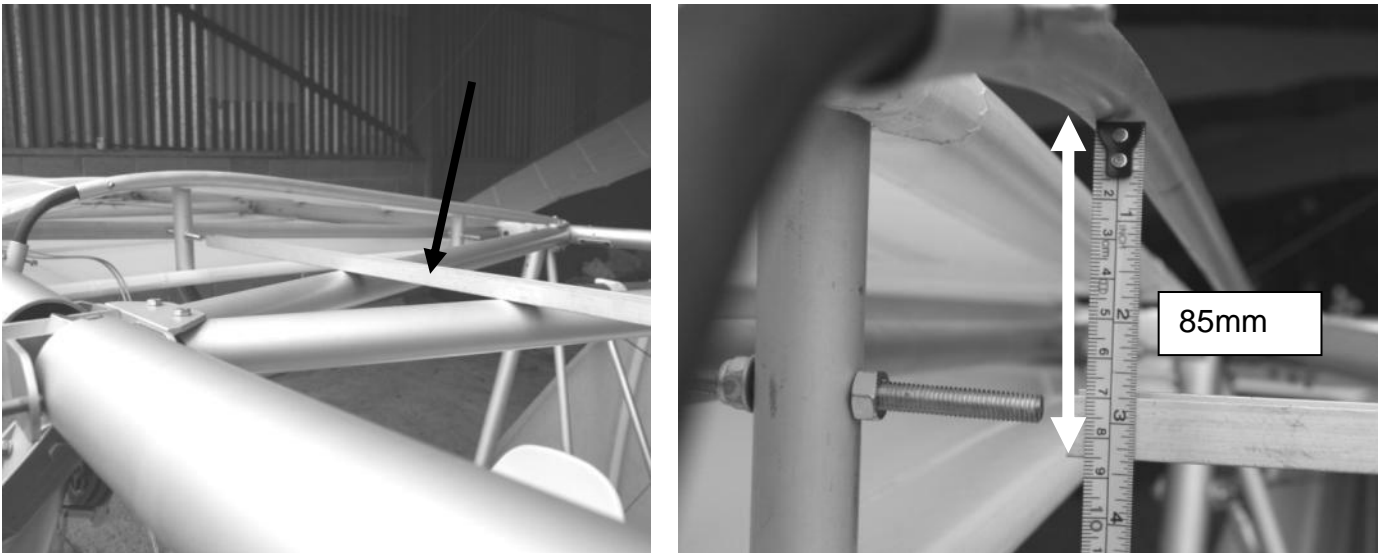
Figure 173 straight edge across cabin upper tubes. Measurement of 85mm from under tube to straight edge at point of max camber
