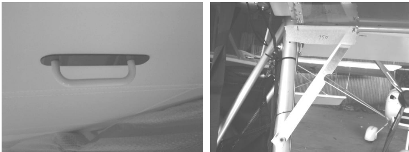
Figure 306 door open keeper, and example of an alternative fabricated stay.
