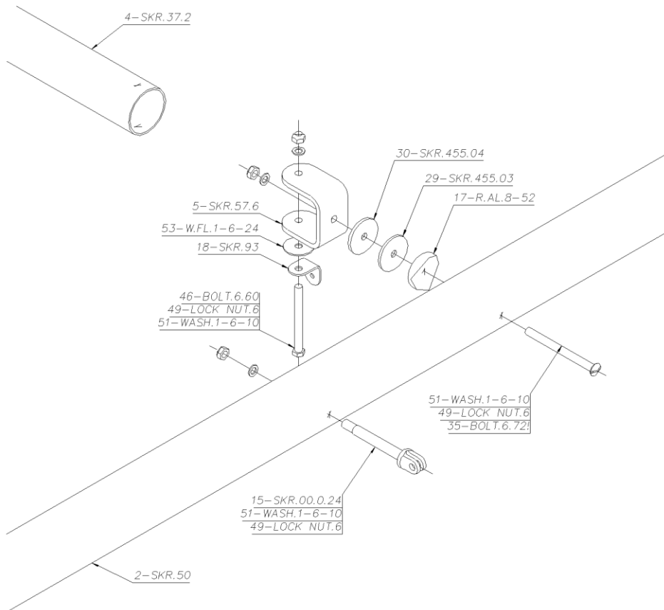
Figure 136 rear jury strut attachment.
