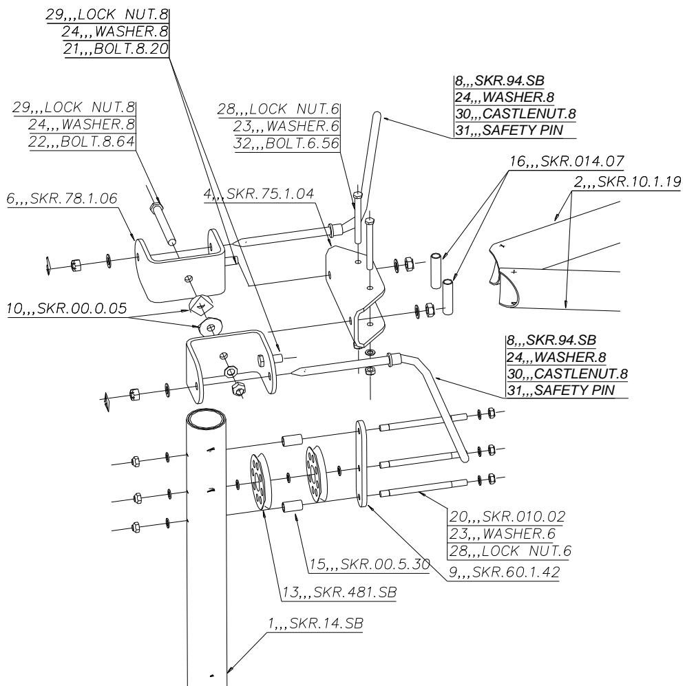
Figure 26 forward end of upper cabin triangle.
