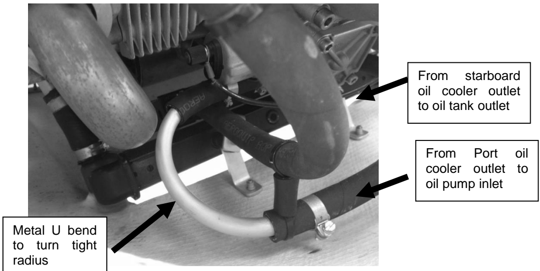
Figure 207 Hose routings from oil cooler outlets
