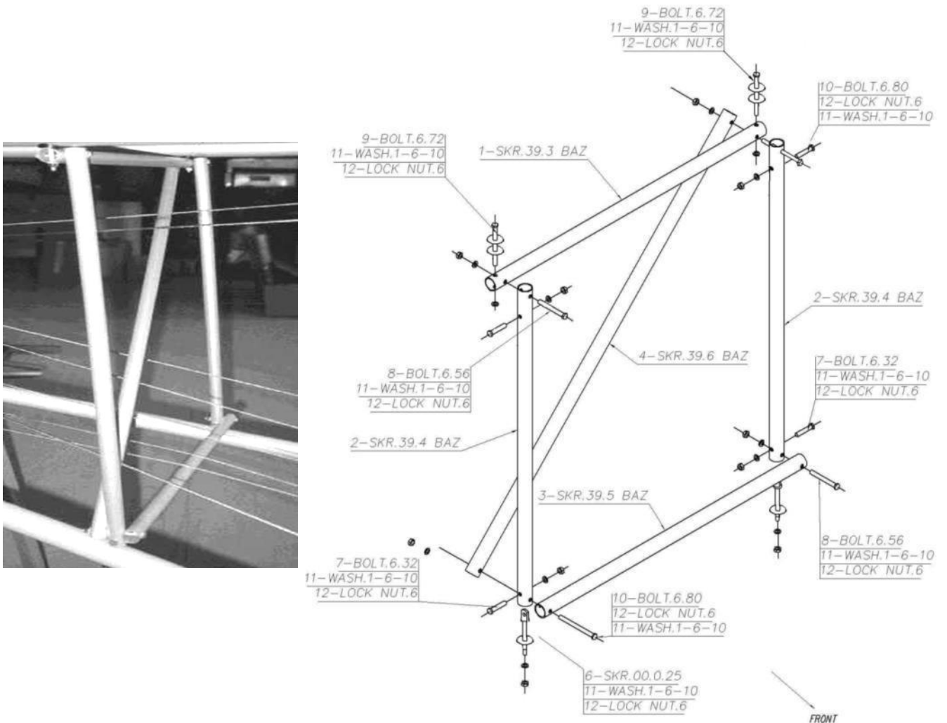
Figure 60 rear fuselage bracing frame. Note orientation arrow.
