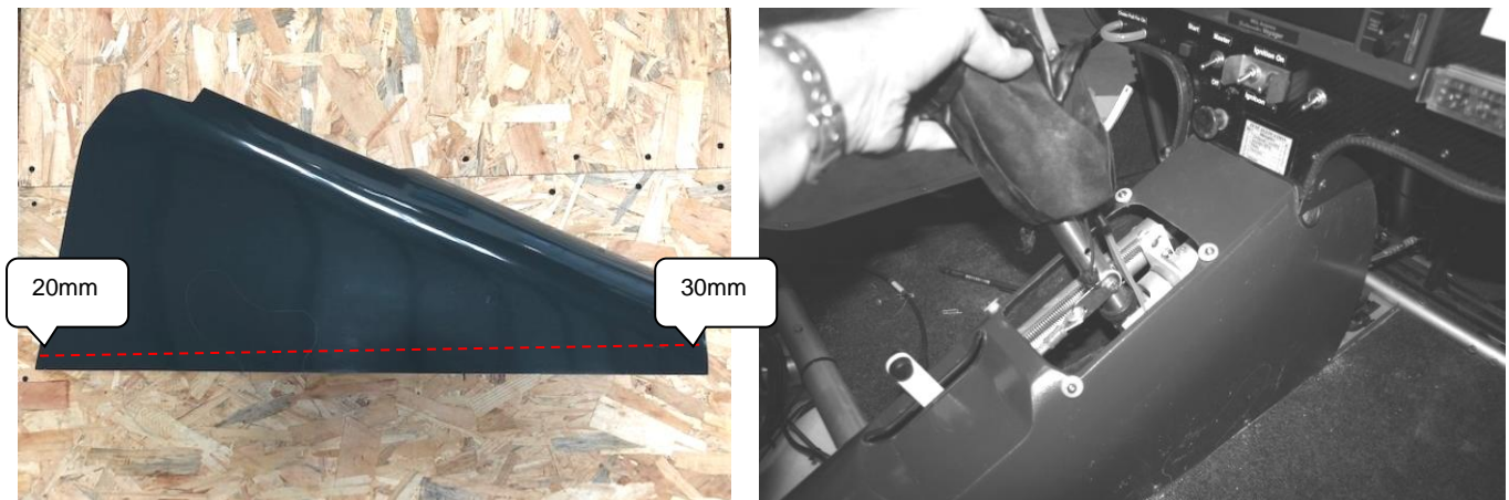
Figure 325 cutting lower edges and stick opening
