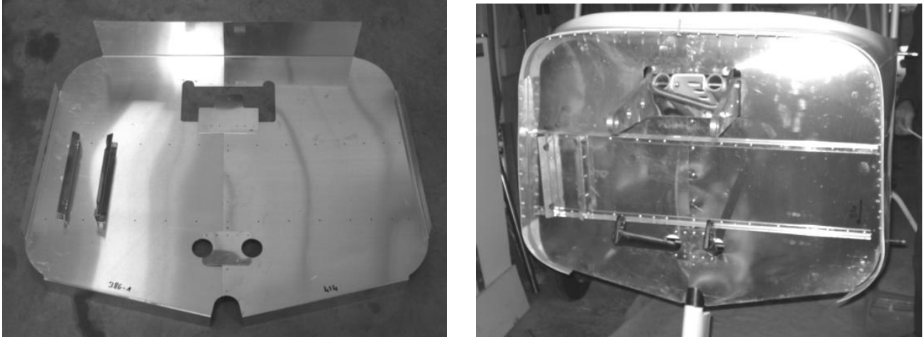
Fig 183 Firewall components, and installed firewall (engine removed for clarity)
