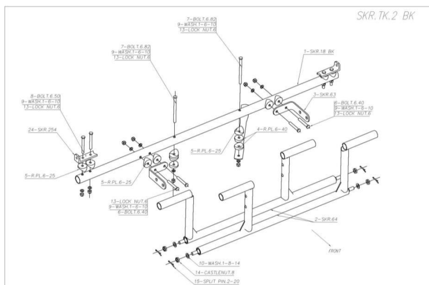
Figure 52 rudder pedals.
