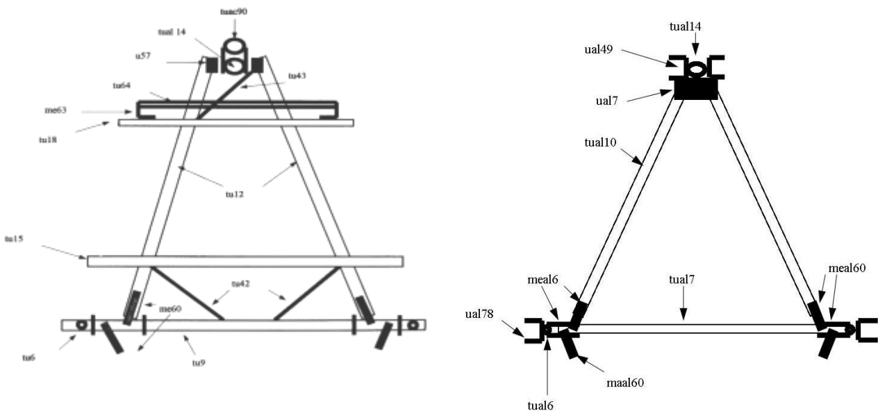
Figure 11 cabin lower and upper triangle tube numbering.
