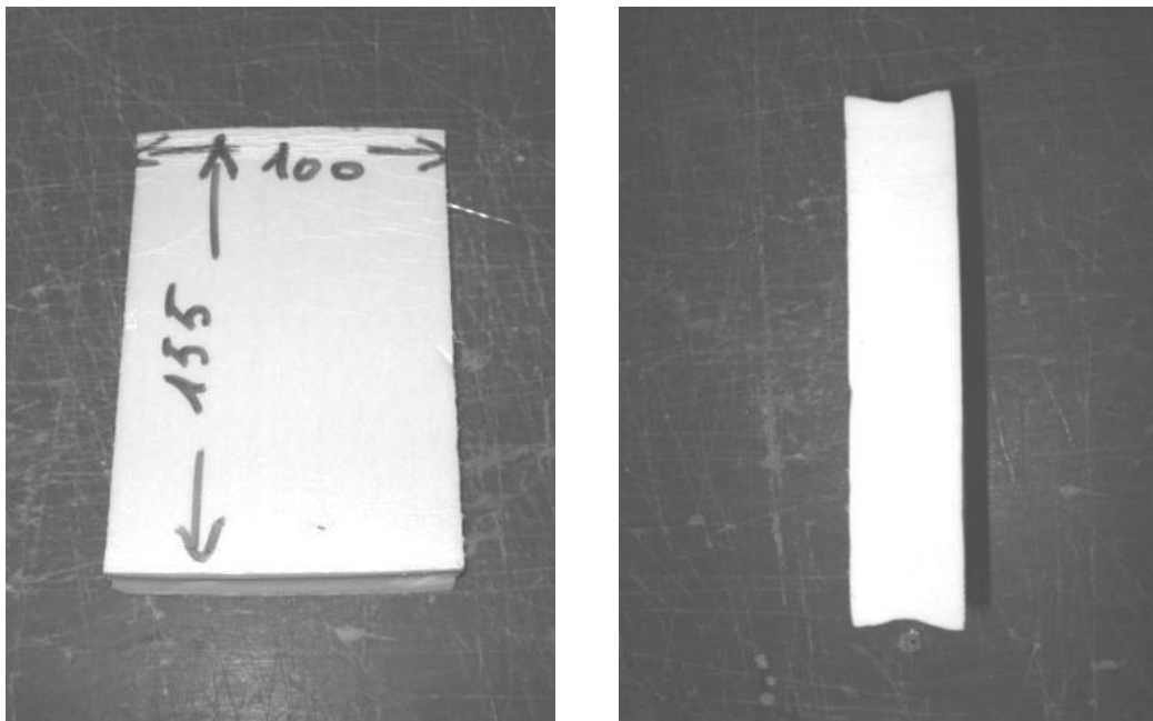
Figure 359 Support block dimensions and grooves
