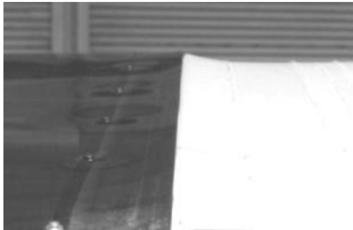
Figure 289 lexan edge matched to wing covering root batten peak
