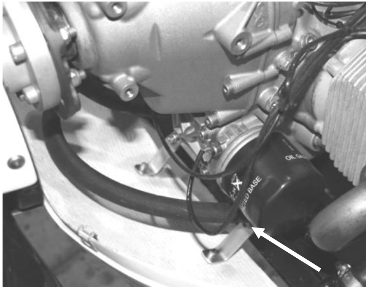
Figure 206 hose should be pulled forwards with cabletie and short standoff in position indicated to provide good clearance from fretting on engine
