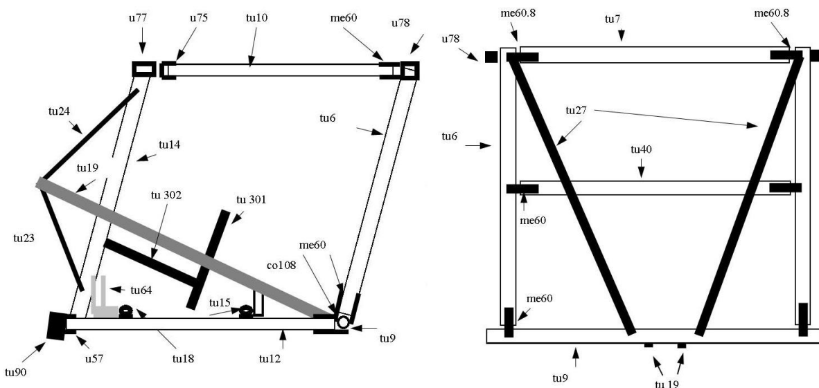
Figure 12 cabin viewed from port side, and rear cabin frame viewed from rear.
