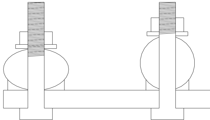
Figure 10 Left - WRONG – squashed tube, thread in tube. Right – RIGHT – tube still round, thread stops in washer(s).
