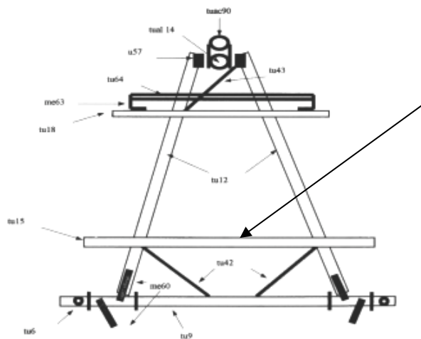
Figure 51 SKR15 seat front support tube.
