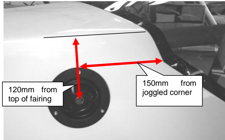
Figure 232 filler location
