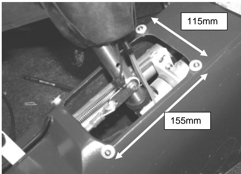
Figure 329 Control stick gaiter fixings.
