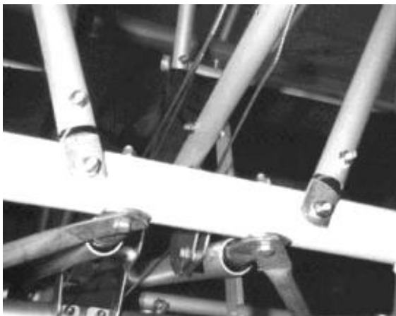
Figure 28 lower and upper ends of rear cabin frame diagonals.
