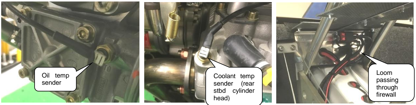
Fig 282 – sender, RPM and ignition loom
