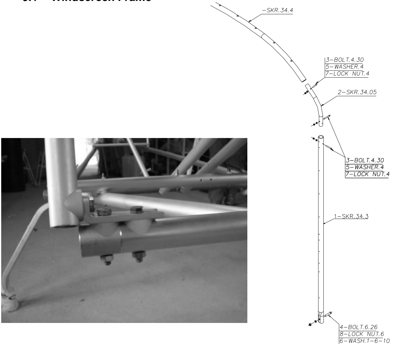
Figure 168 cabin uprights ( note that saddle washer shown may be superseded by flattened tube sides and 1mm plastic washer should then be used).
