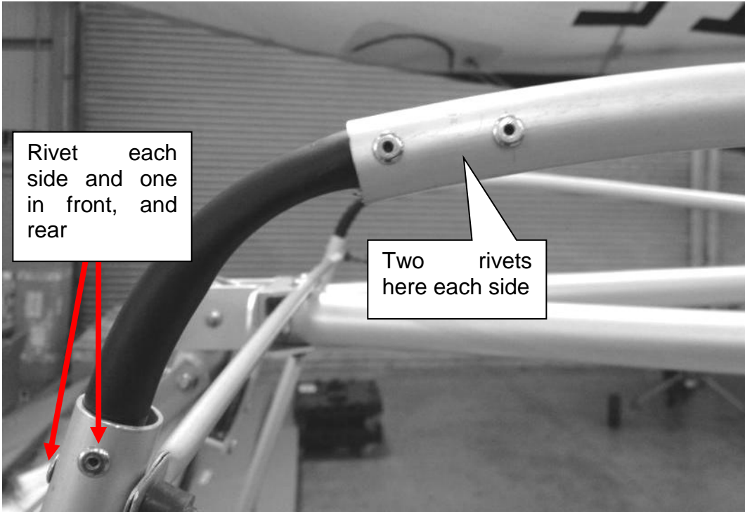
Figure 172 – stabilising with rivets
