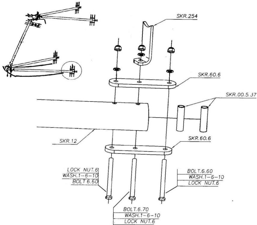
Figure 17 lower cabin triangle, rear of tube SKR.12 (note, find SKR254 in assembly bag A9)
