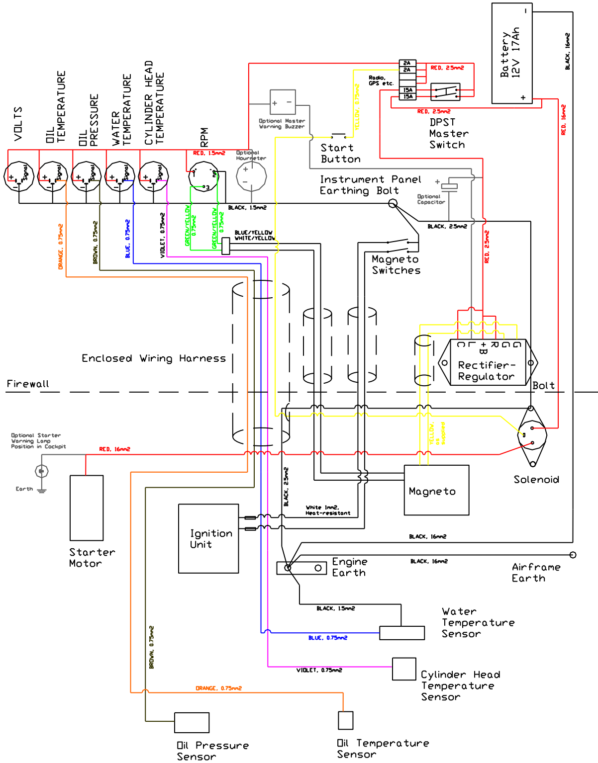
Figure 276 overall wiring schematic, Rotax 912 and standard analogue instruments. (ensure all colours are visible when printed out)
