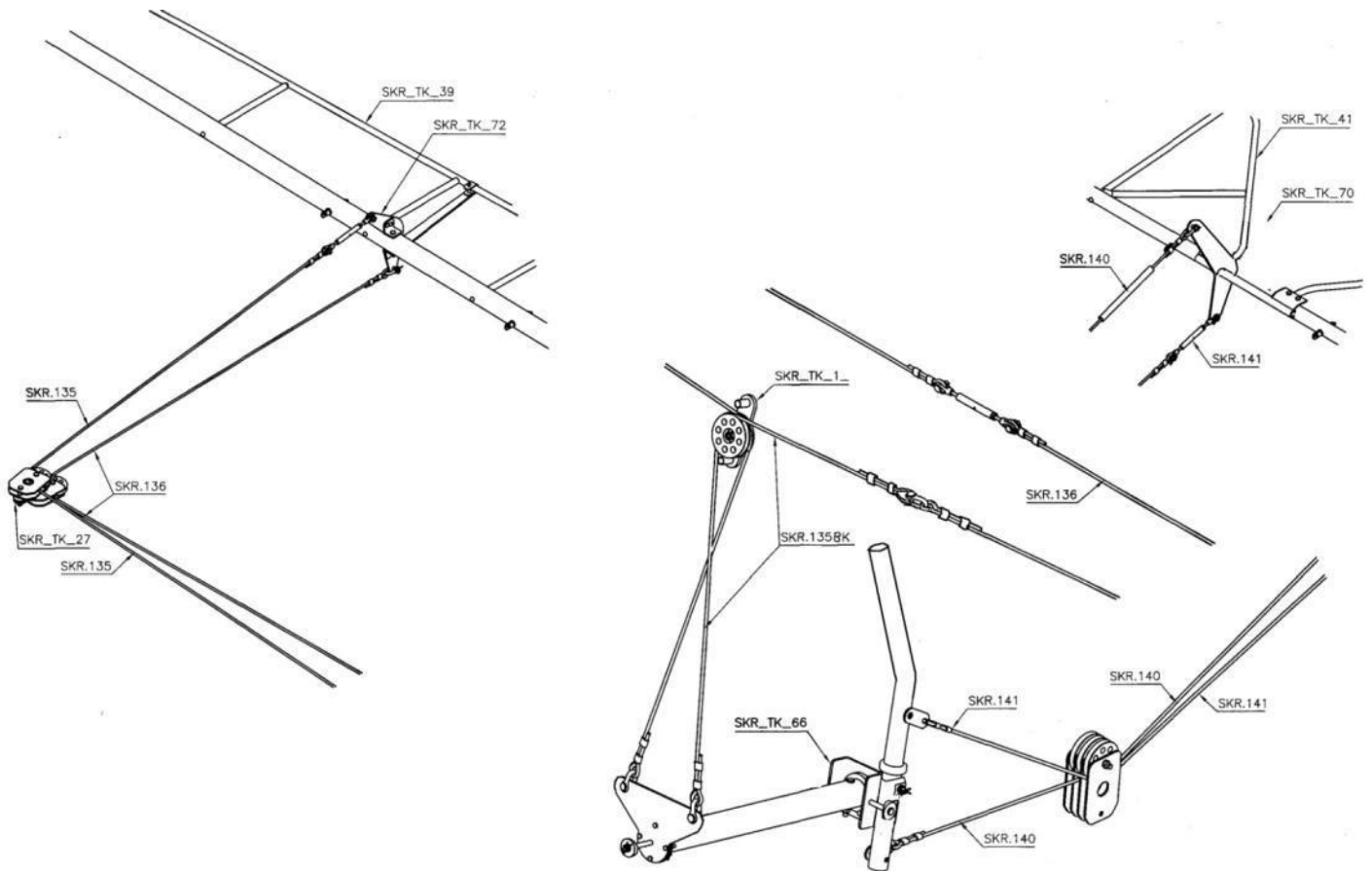
Figure 147 aileron cable runs.
