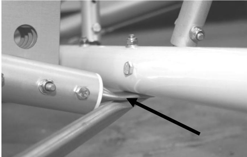
Fig 38 Rear of SKR19 – ends must be bent to align like his
