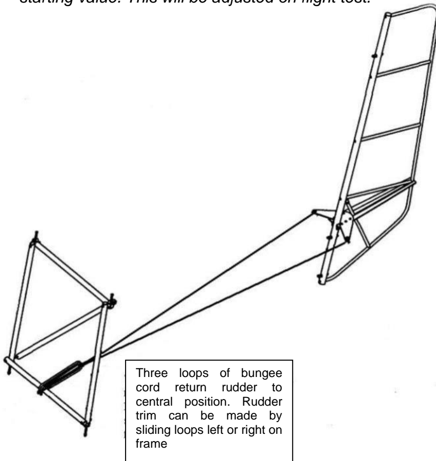
Figure 111 rudder centering bungee arrangement
