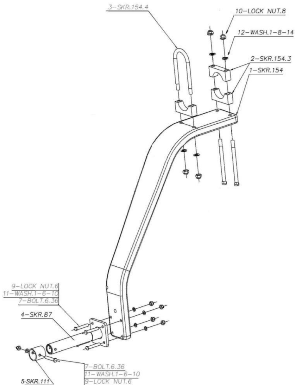
Figure 79 Nynja undercarrige leg
