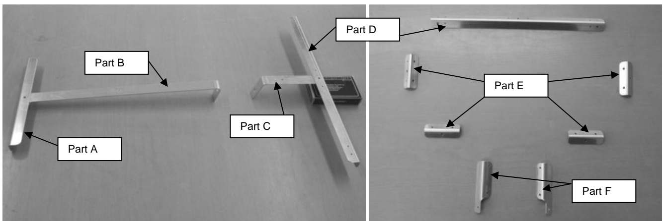
Figure 235 dashboard supports and instrument panel framing angles
