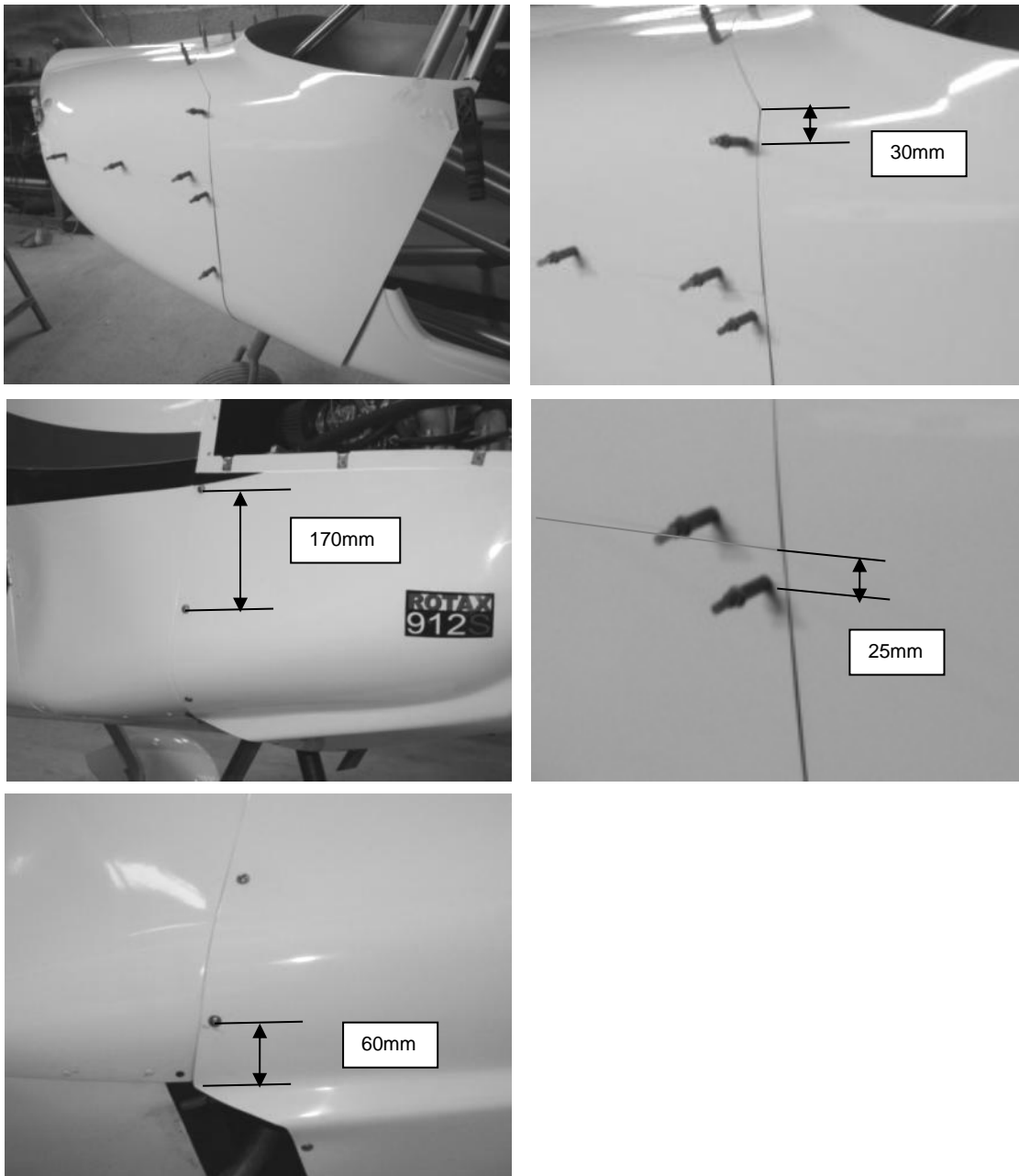
Figure 191 fixing the cowlings to the scuttle (note cowling may now be supplied with moulded vent holes in lower sides, adjust position of fixing holes accordingly).
