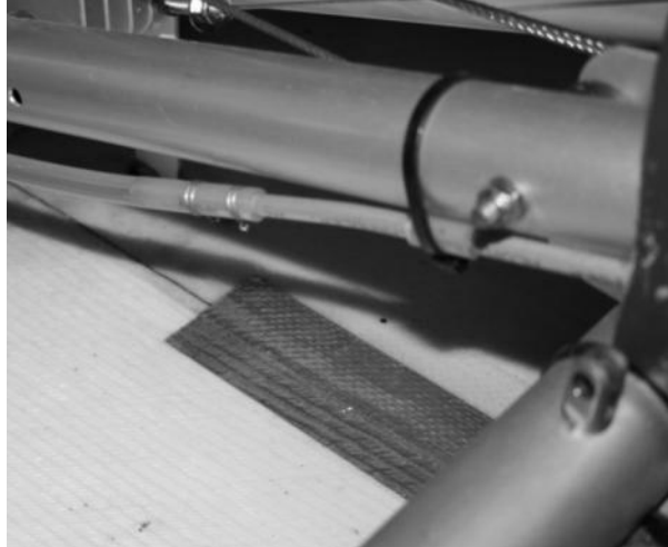
Figure 218 aluminium fuel line, cable tie and standoff.
