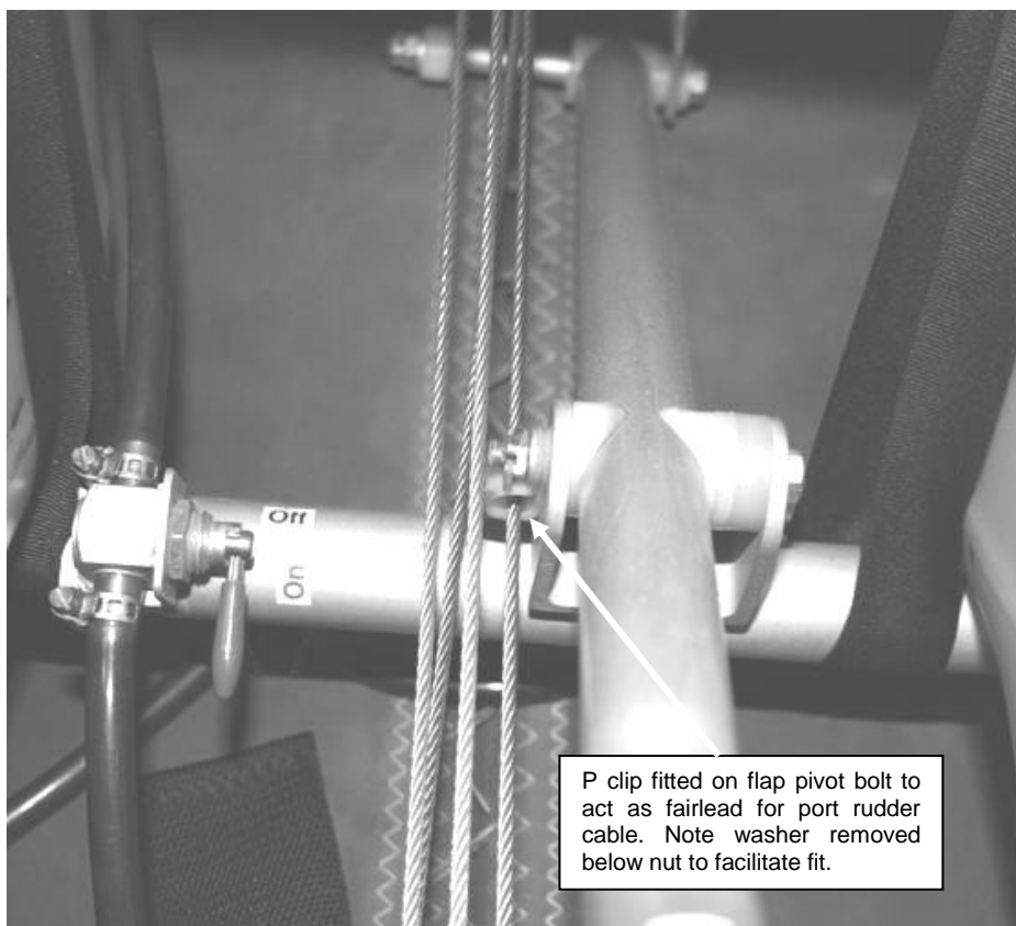
Figure 110 Port rudder cable fairlead
