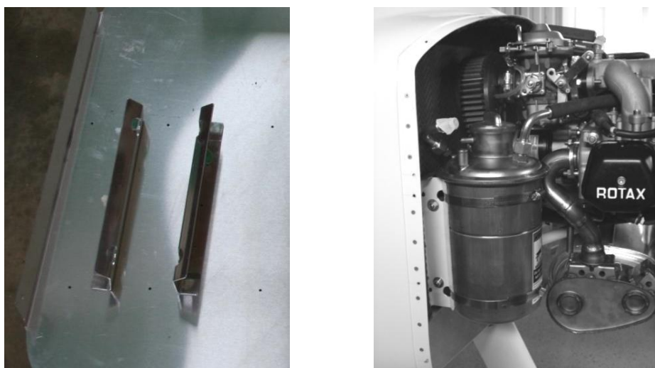
Figure 201 Oil tank mounting
