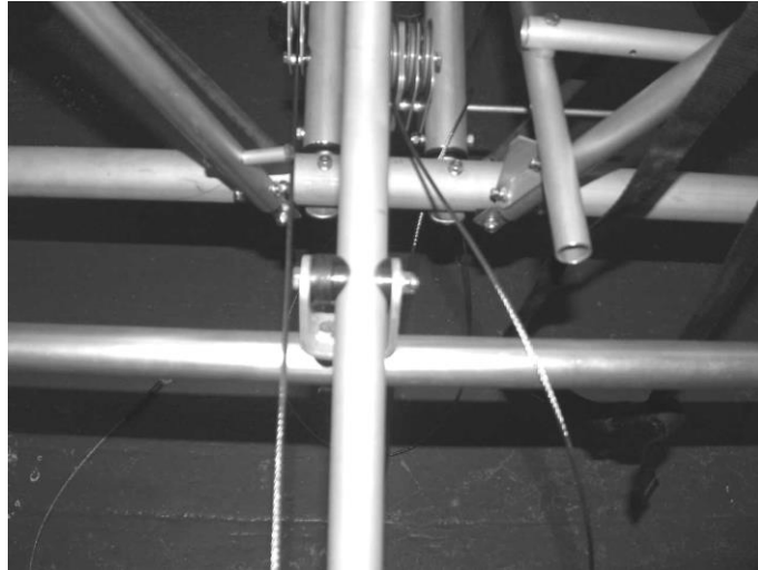
Figure 71 flap handle pivot.
