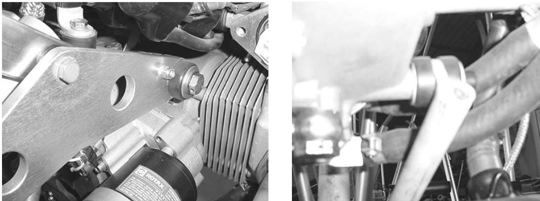
Figure 127 upper starboard and lower port mounting bolt.
