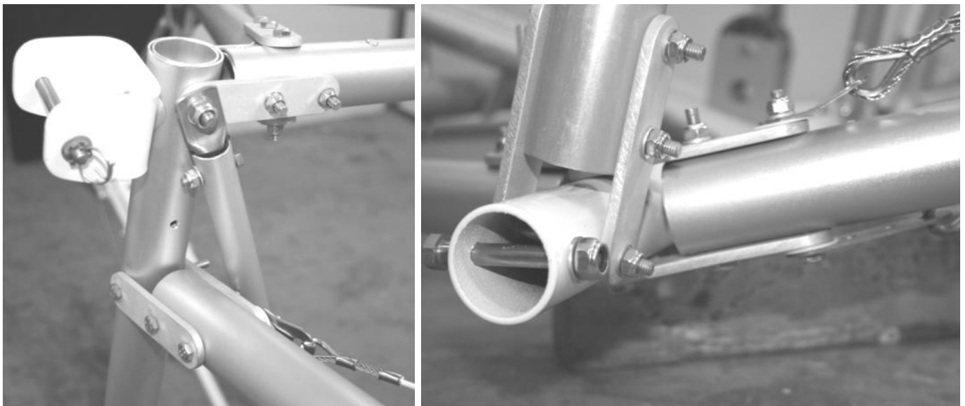
Figure 62 forward ends of upper and lower tubes
