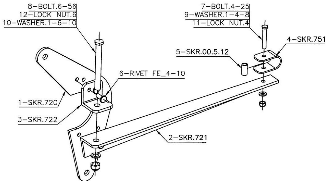
Figure 143 aileron horn parts.
