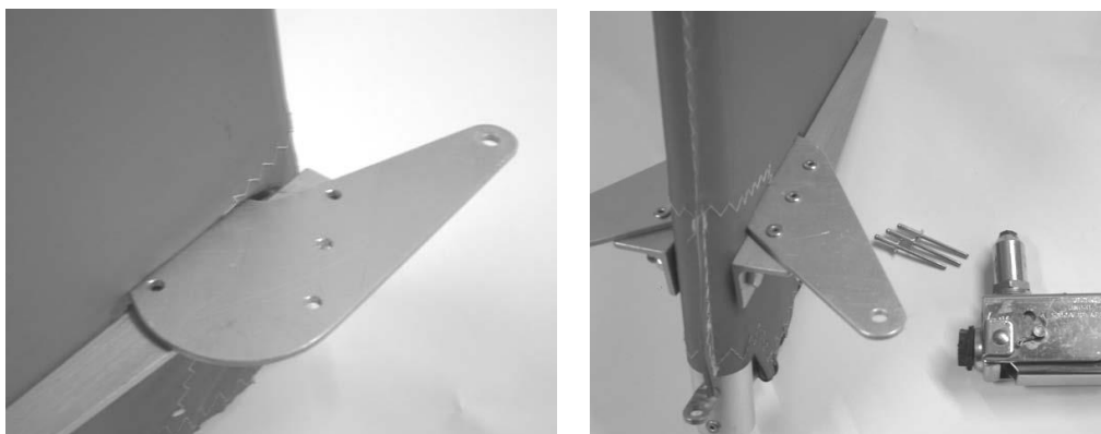
Figure 102 rudder horn fixing.
