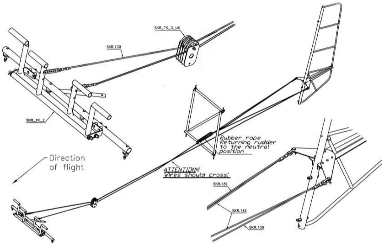
Figure 106 Rudder cable schematic
