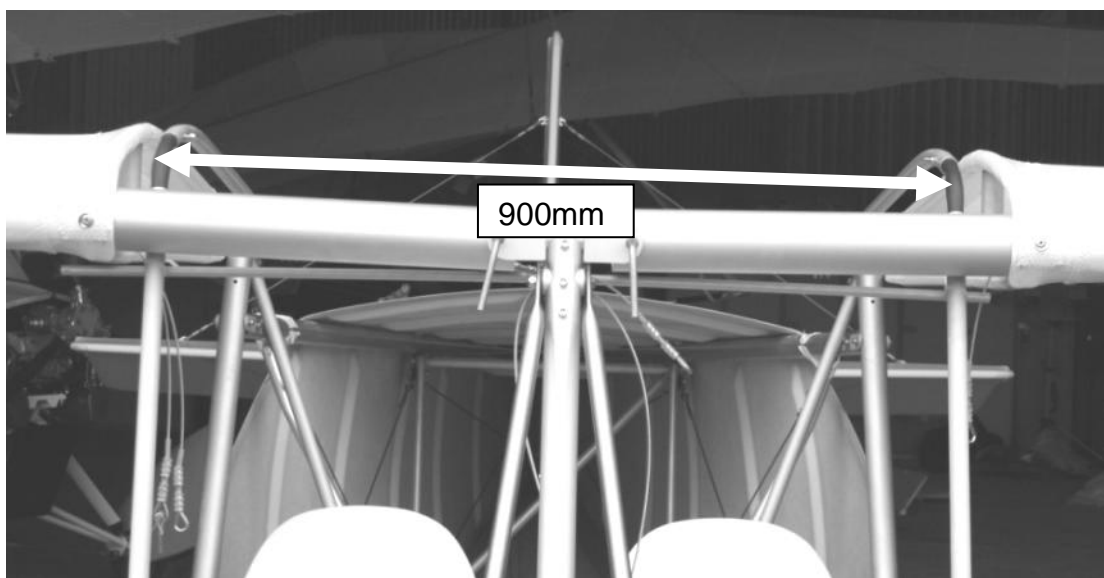
Figure 170 Position TU34 uprights 900mm apart
