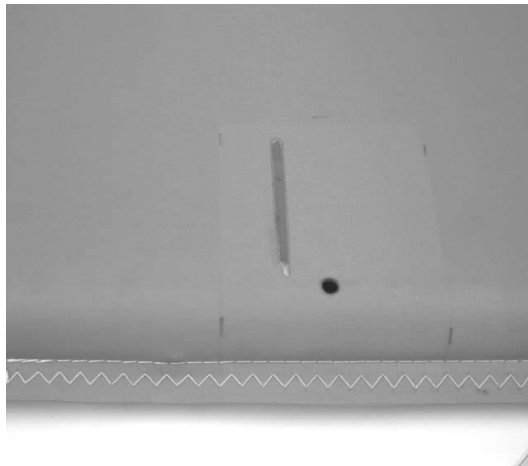
Figure 145 slot for the aileron horn in the under surface of the aileron,
