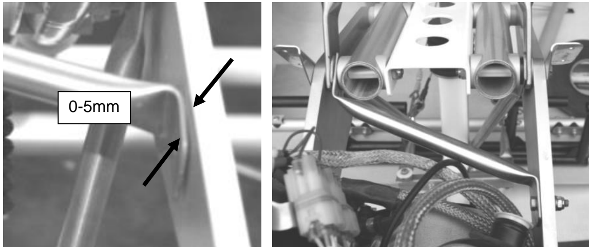
Figure 46 fixing position for TU310
