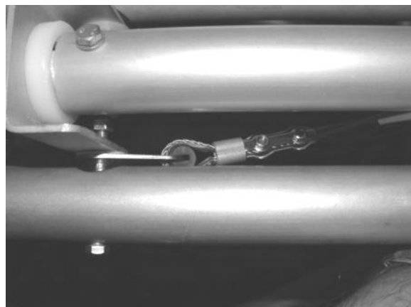
Figure 113 rudder stop cables attached to rear stick pivot.
