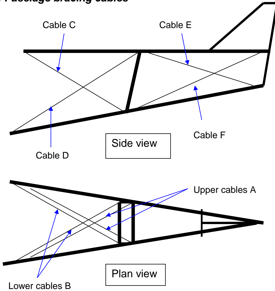
Figure 63 fuselage cable arrangement overview
