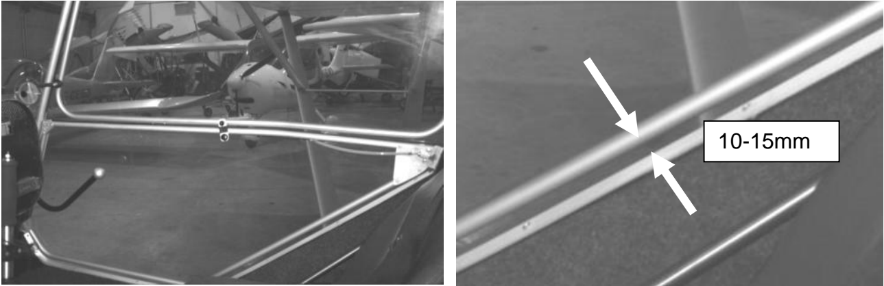
Figure 309 tube spacing
