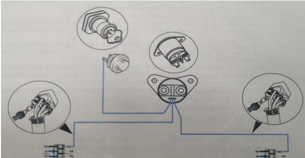
Figure 280 – 'Easy start' wiring diagram
