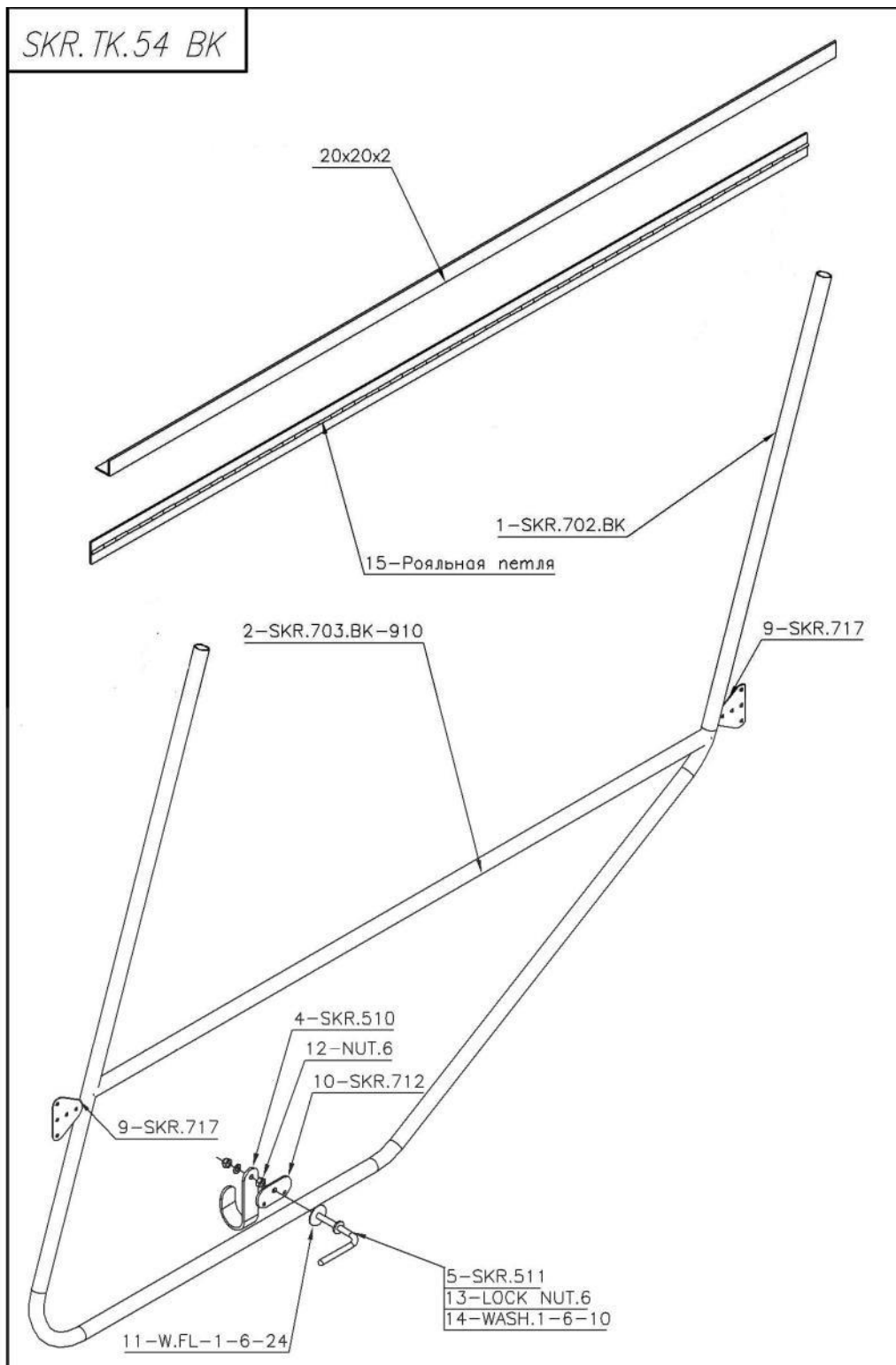
Figure 299 one piece door frame.
