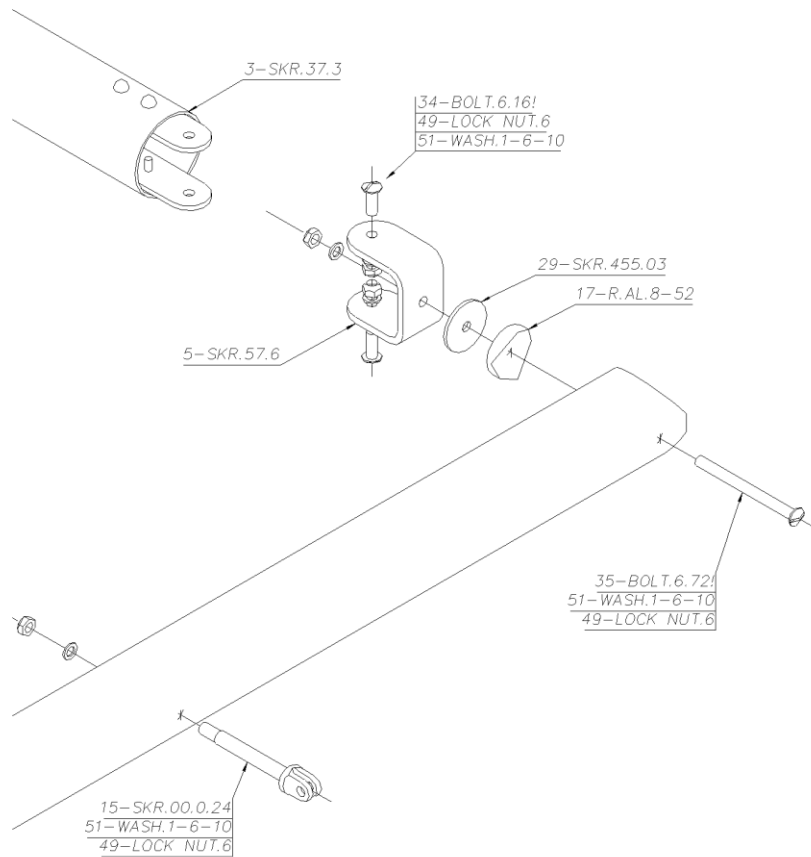
Figure 132 rear of tip.
