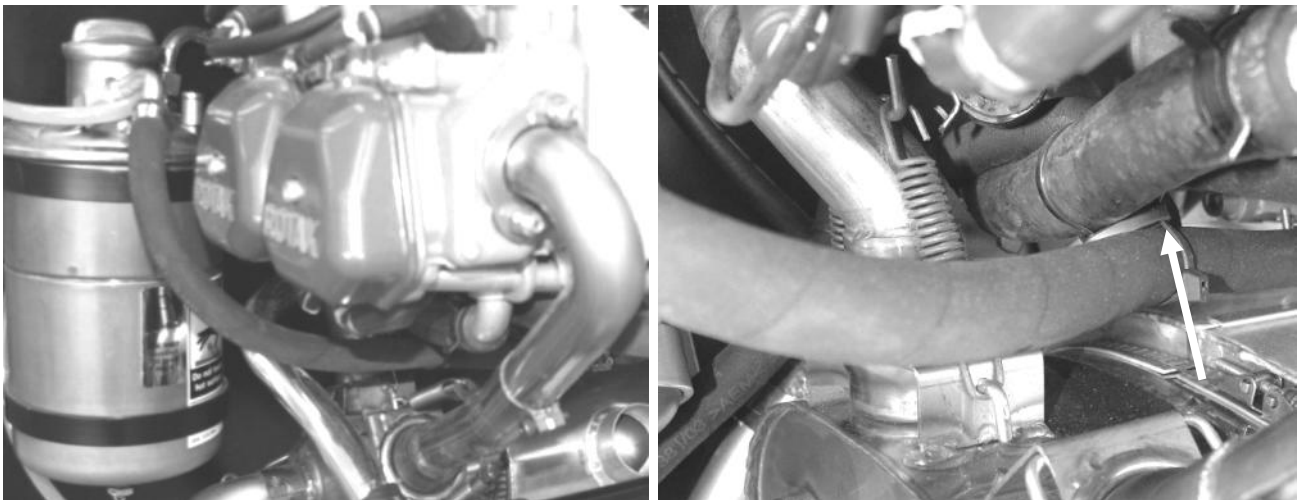
Figure 208 Routing of oil hose from Sump connection to inlet of oil tank. It should be cabletied up to the small water pipes under the engine in the position marked to keep it clear of exhaust.
