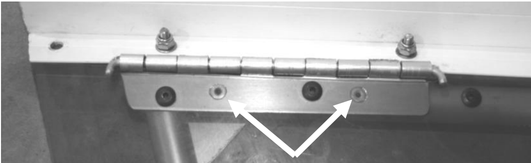
Figure 315 top rail tube fixed to hinge
