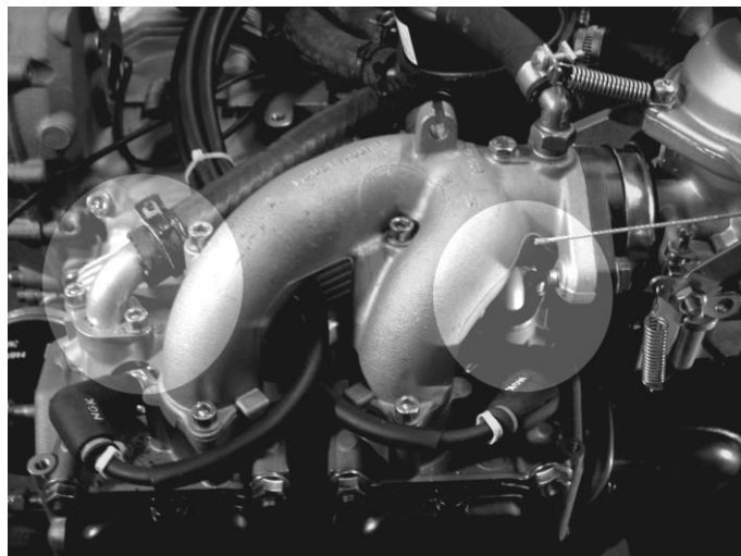
Figure 210 water pipe attachment elbows to left of, and under, inlet manifold.
