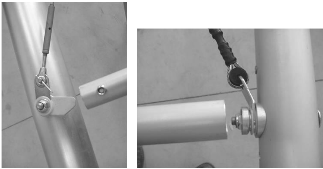
Figure 142 tensioning tube fittings, front in left photo (note bolt through compression tube), rear in right photo.
