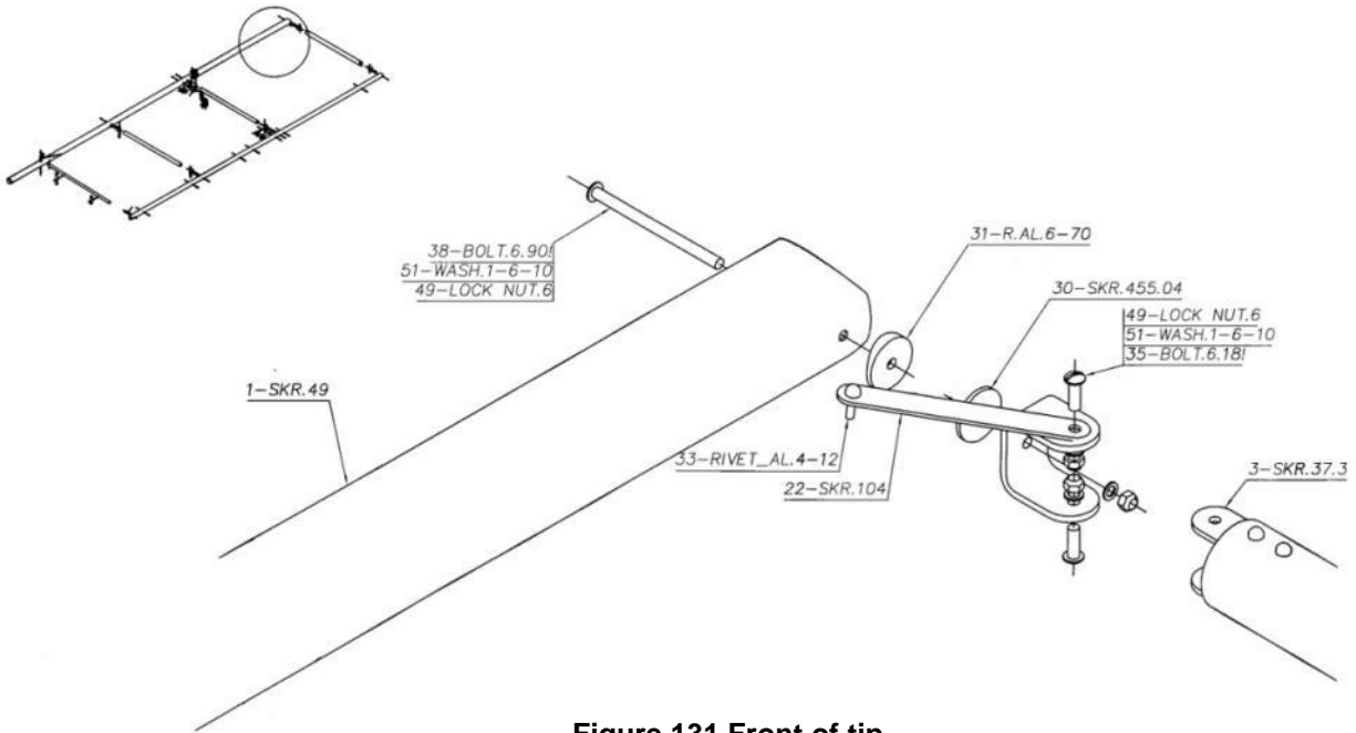
Figure 131 Front of tip
