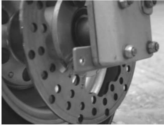
Figure 80 main gear inner spat mount.
