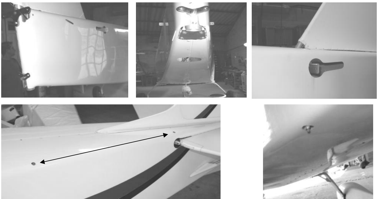
Figure 116 fairing cutouts
