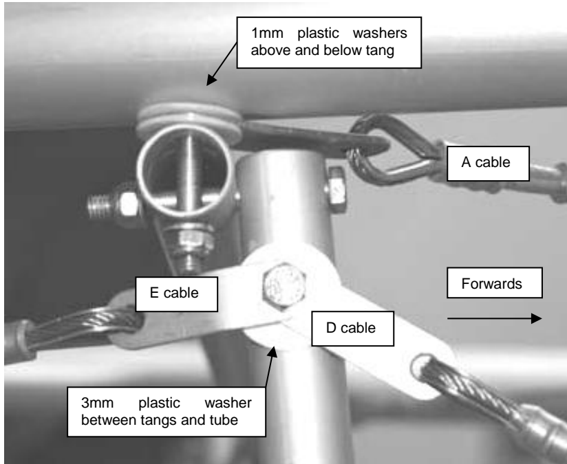
Figure 66 cable arrangement Upper starboard side of central frame
