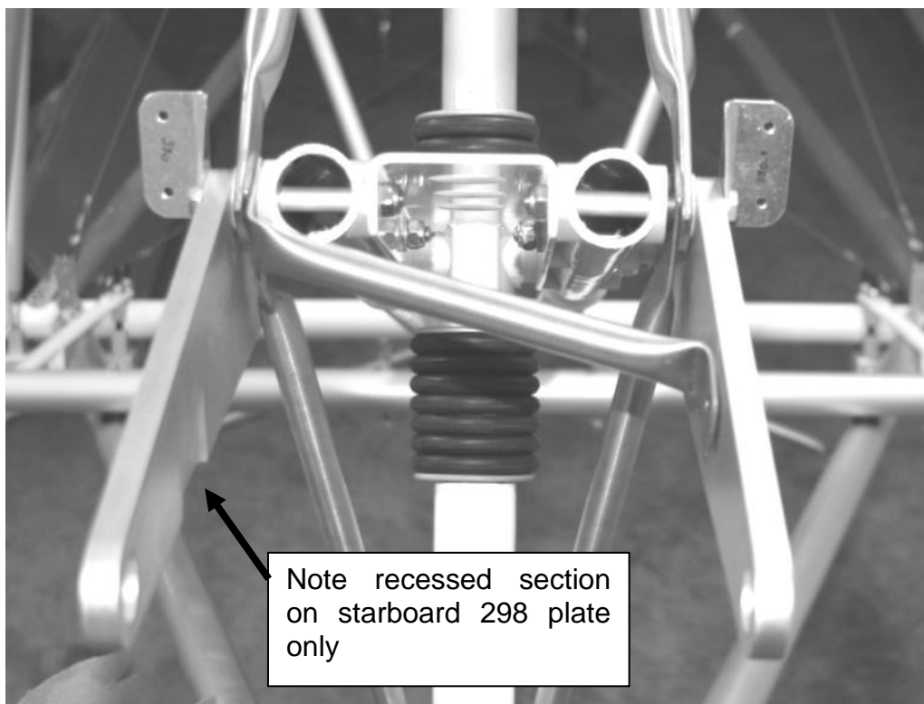
Fig 39 handing the 298 plates
