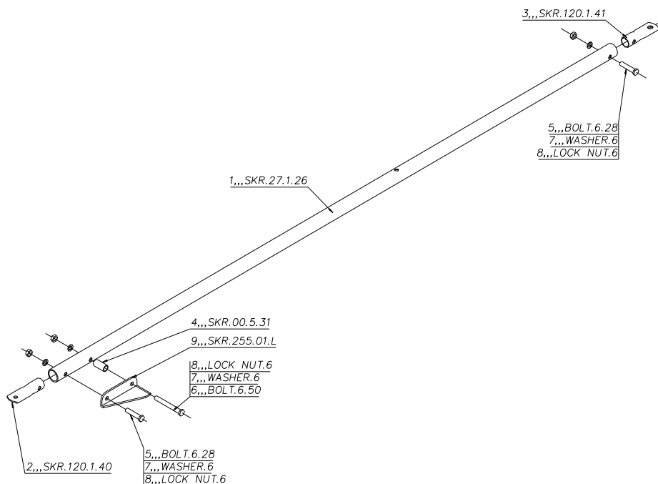
Figure 30 rear cabin frame diagonal, port side viewed from rear.
