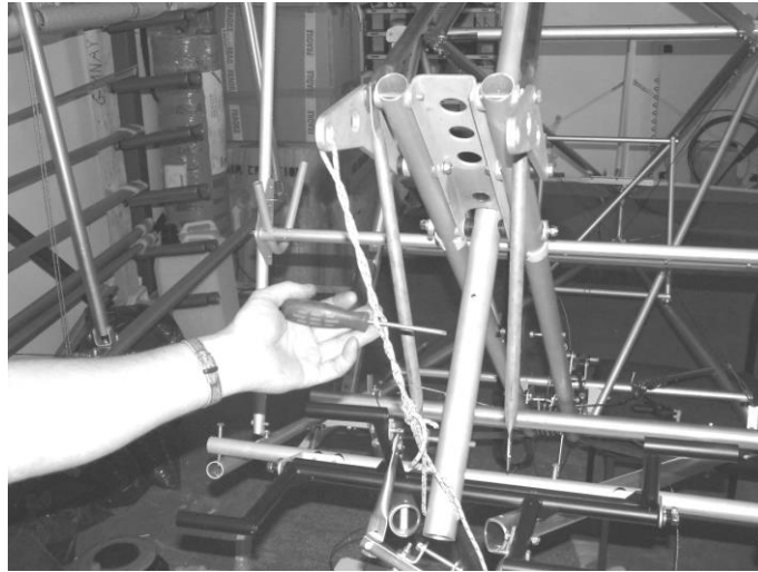
Figure 44 twisted rope used to pull down on engine mount.
