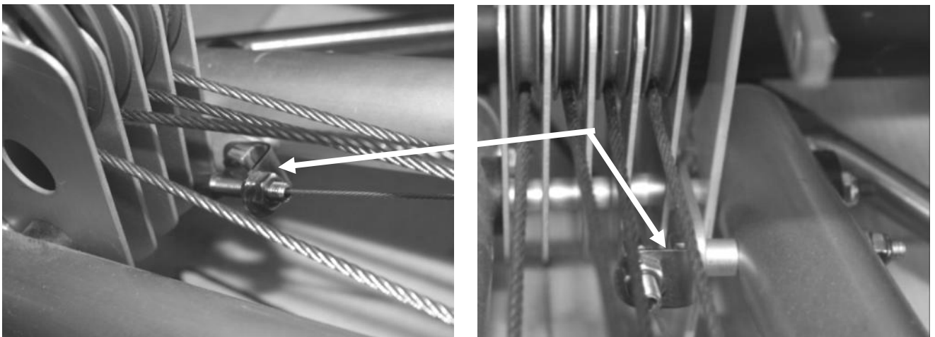
Figure 316 trim tab forward cable bracket
