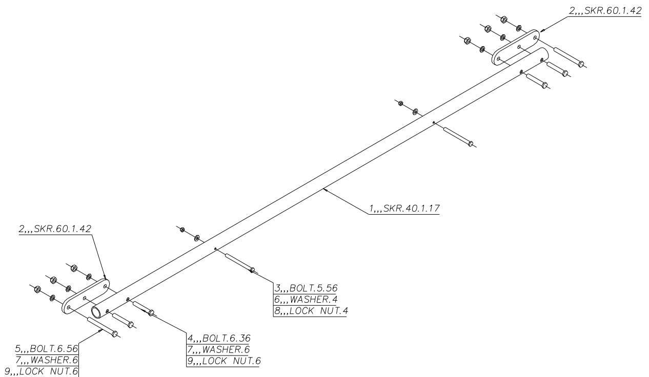
Figure 31, tu40, rear cabin frame cross-piece, looking from the front.
