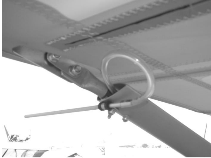
Figure 275 Pitot probe location.
