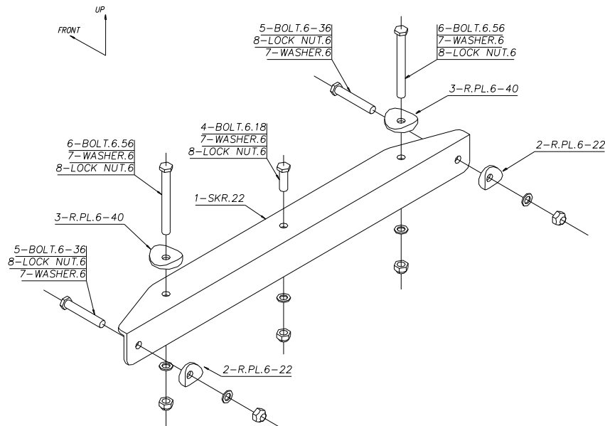
Figure 97 vertical and horizontal stabiliser front mounting.
