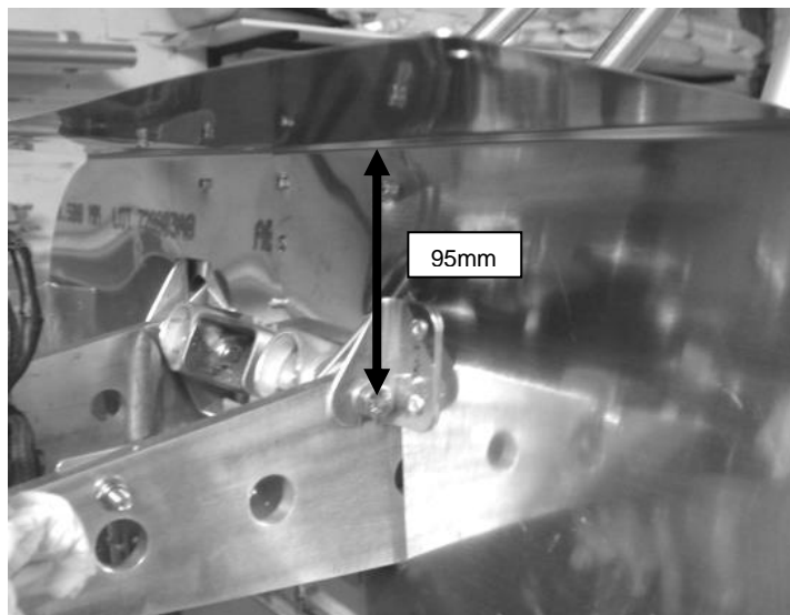
Figure 184 position and fixing of firewall to engine mount
