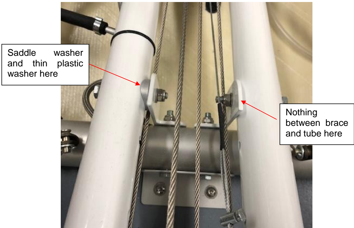
Figure 56 central bracing pieces.
