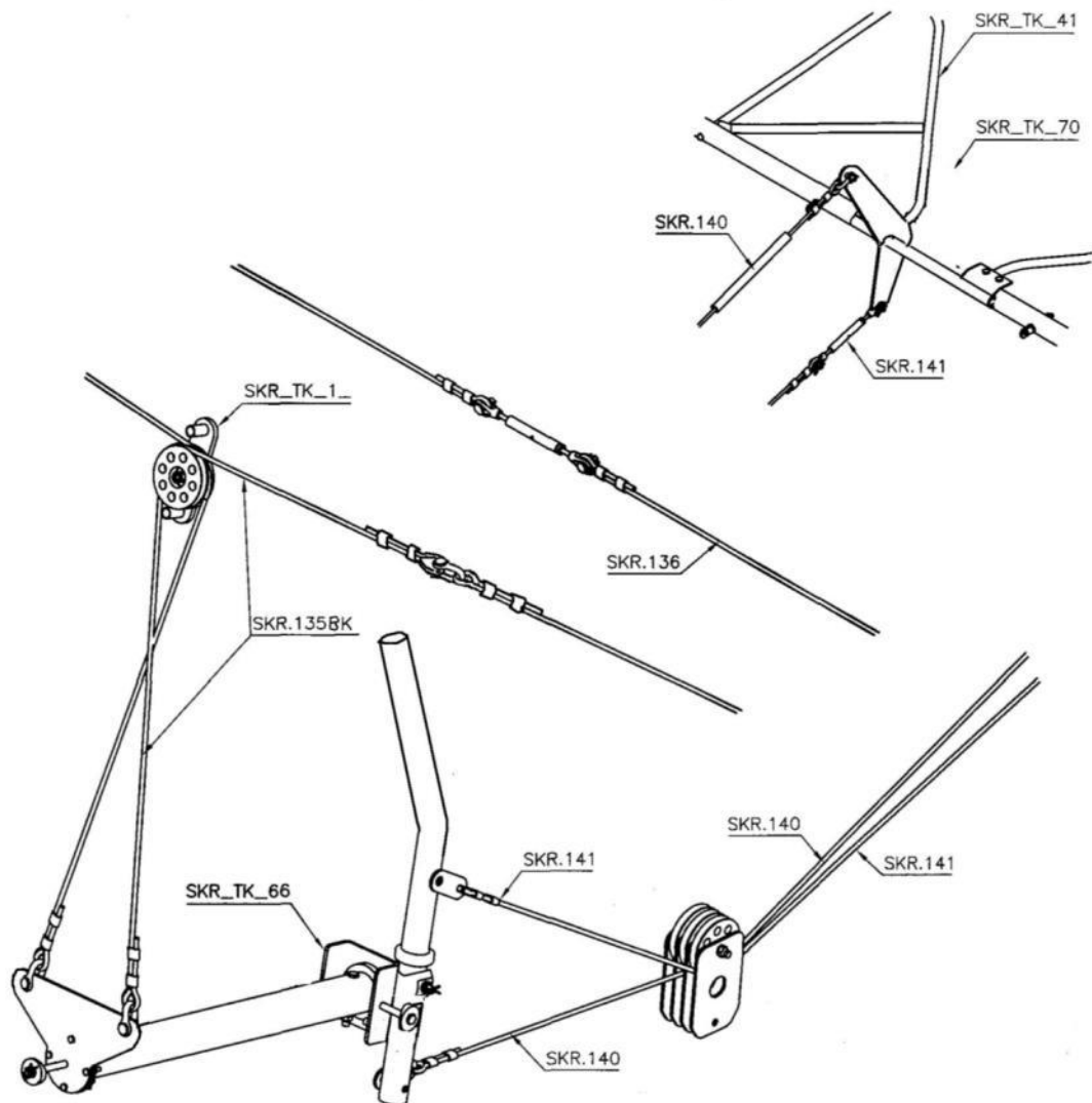
Figure 105 Elevator cable schematic
