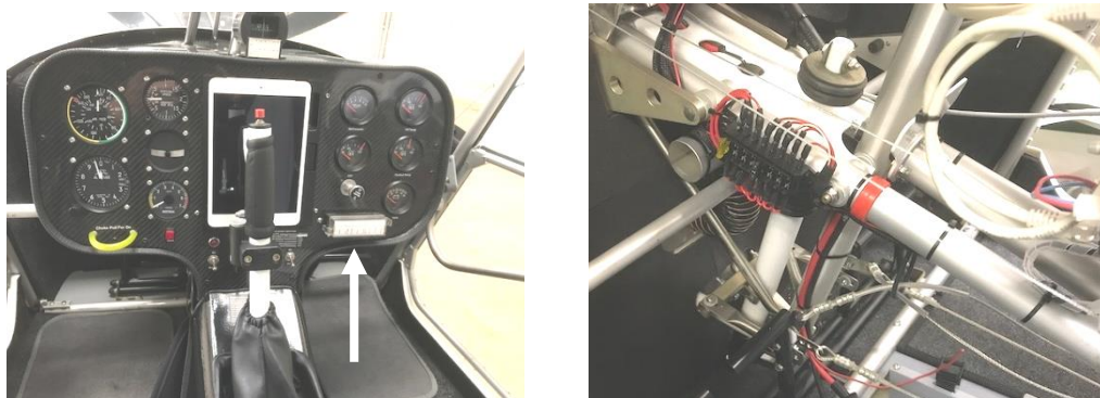
Figure 283- fuse box positions (note right hand picture shows fuse box of different type with connectors exiting sideways).
