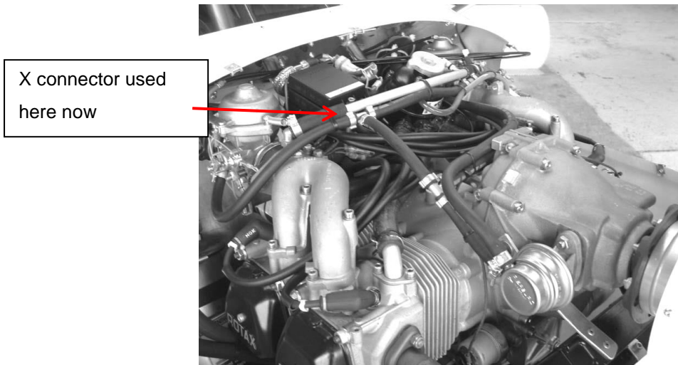
Figure 217 fuel pipe routing in engine compartment.
