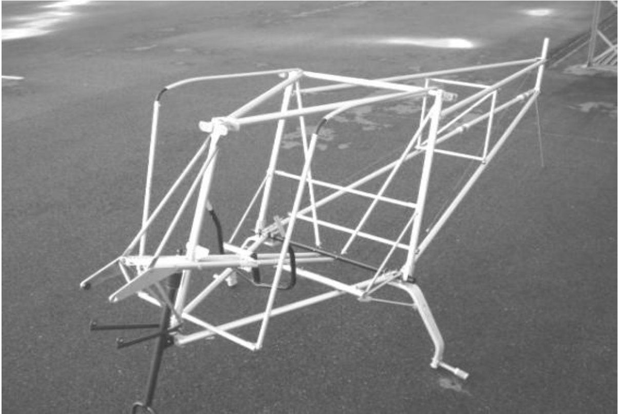
Figure 4 Uncovered Nynja frame
