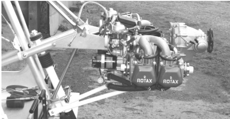
Fig 123 engine installation overview
