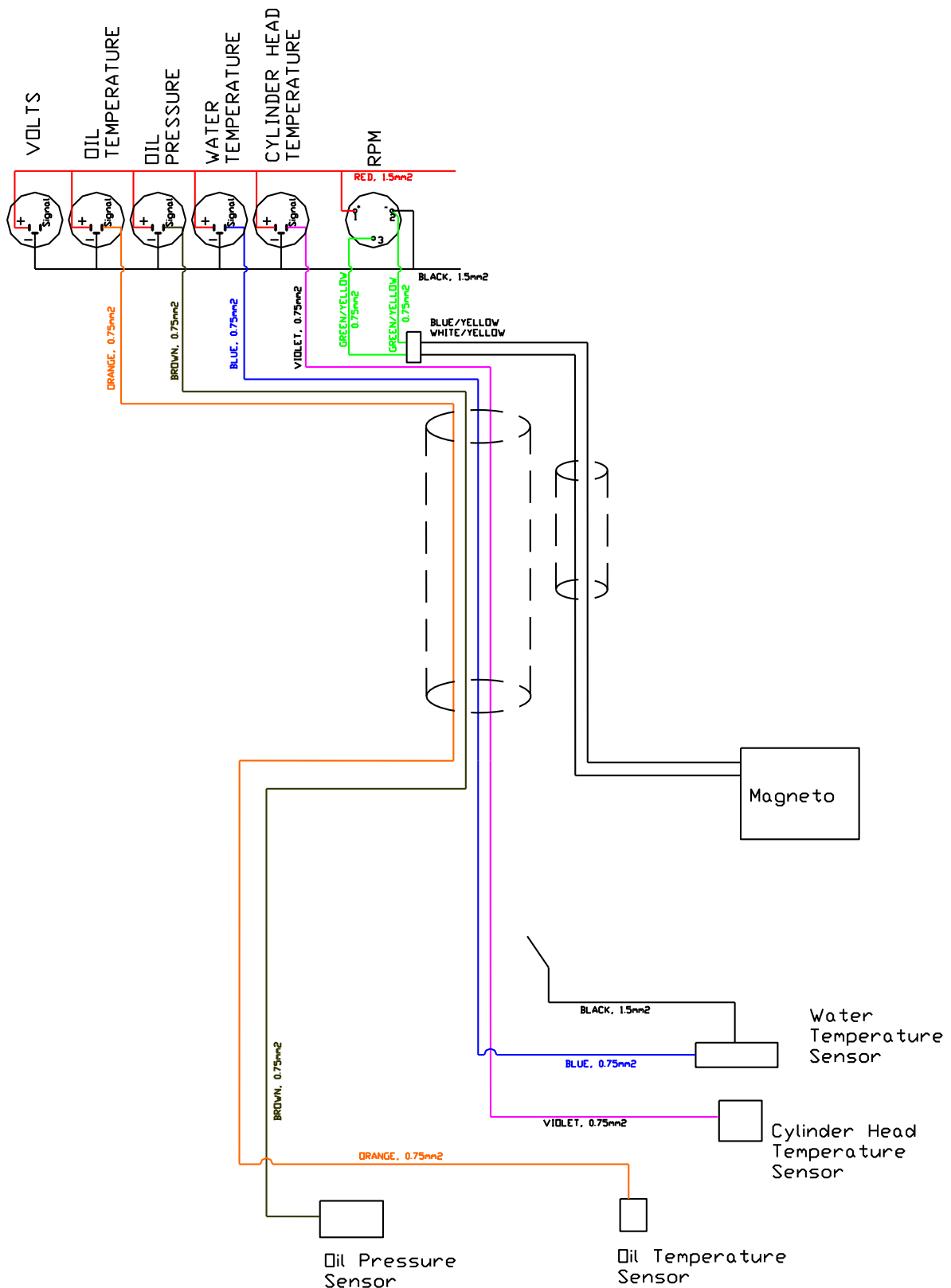
Figure 279 instrument wiring schematic, Rotax 912. (note that later engines have 'wet' temp senders on cylinder heads and what was previously CHT measurement is now coolant, and separate coolant temperature gauges are not required. Also latest wiring looms in the engine installation package include magneto (ignition) wires, and RPM within the made up loom, but Oil pressure is a separate loom).
