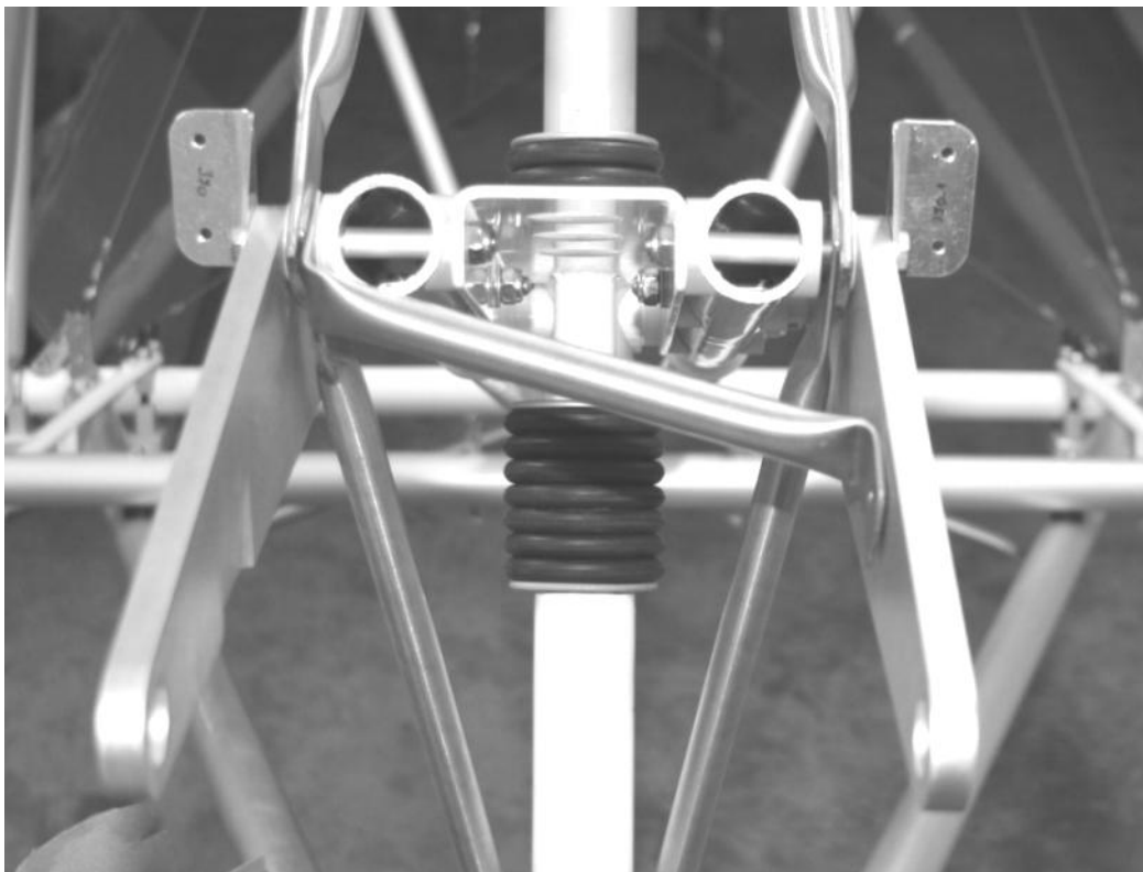
Fig 35 Nynja engine mount assembly
