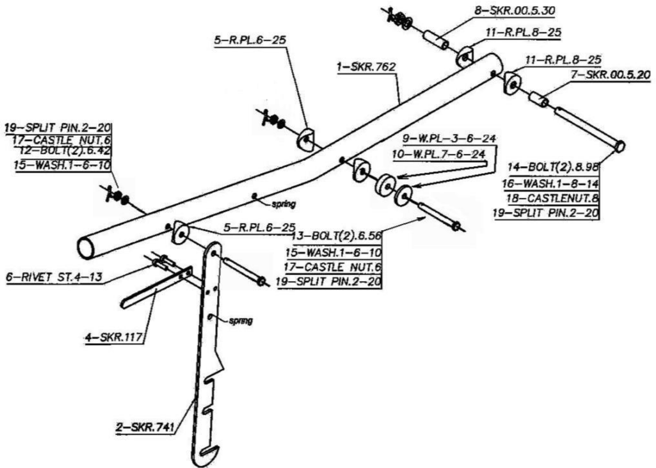
Figure 73 Flap handle
