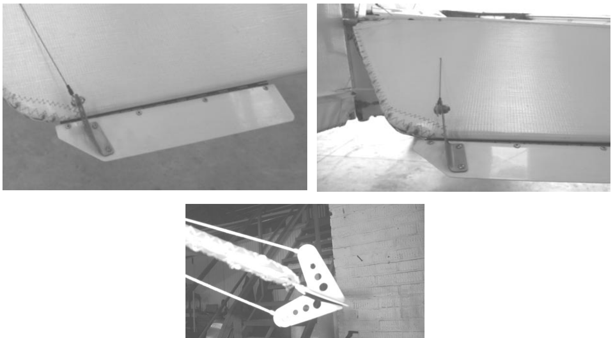
Figure 94 Trim tab horns aligned with cable bracket and hinge pin
