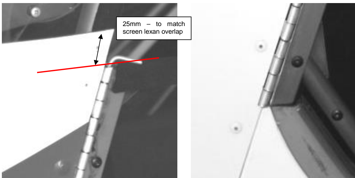
Figure 308 upper and lower hinge positions
