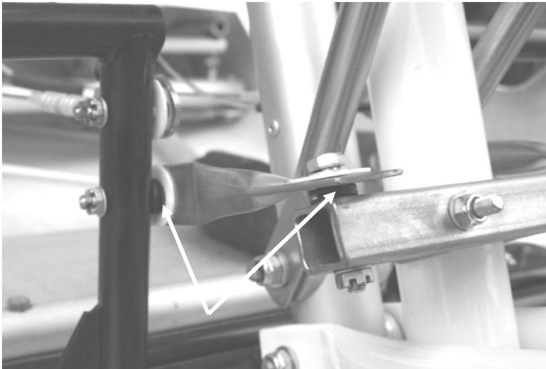
Figure 87 nose wheel steering bar, with rubber grommets between pushrods and box section and pushrods and rudder pedals, note the white plastic washers shown near the arrows should not be fitted.
