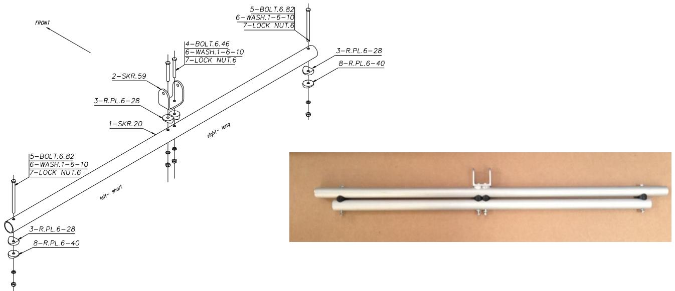
Figure 69 fuel tank support / flap handle mount – M version left – LS version on right.
