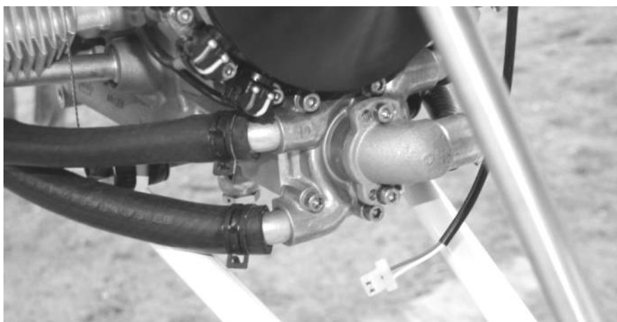
Figure 124 water pump outlet in correct position
