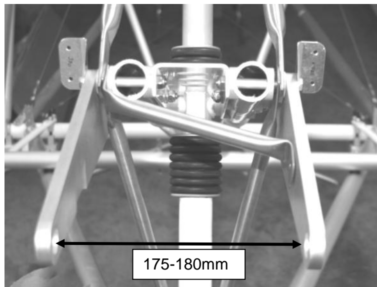
Figure 45 Rotax 912 engine mounts, front view.
