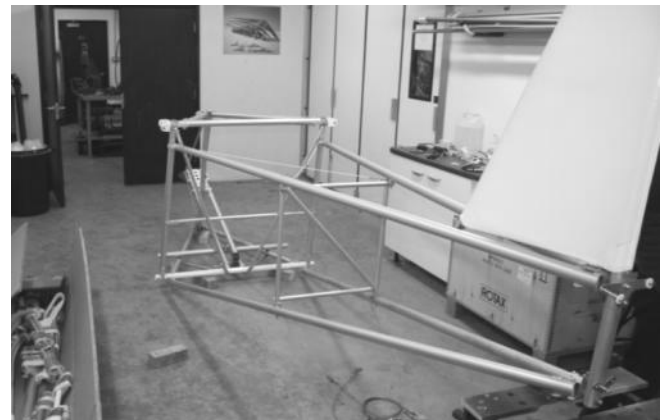
Tailcone fitted to cabin
