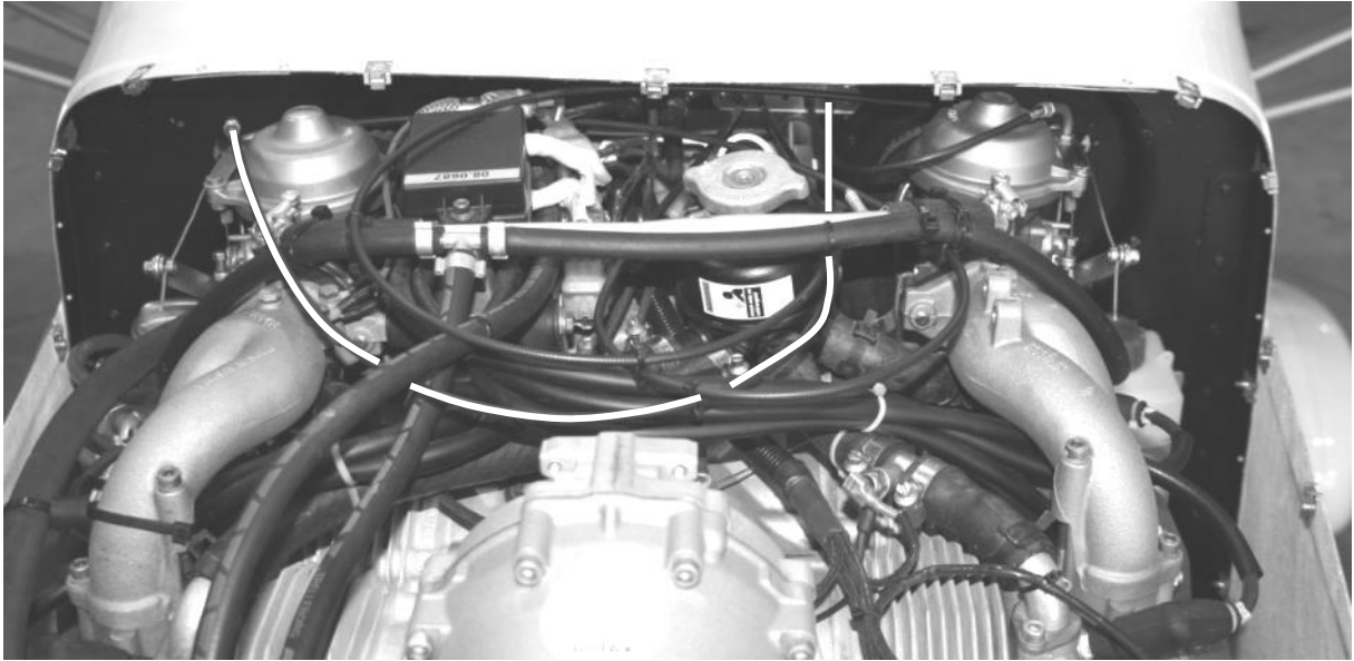
Figure 270 choke cable route to starboard carburettor (in white)
