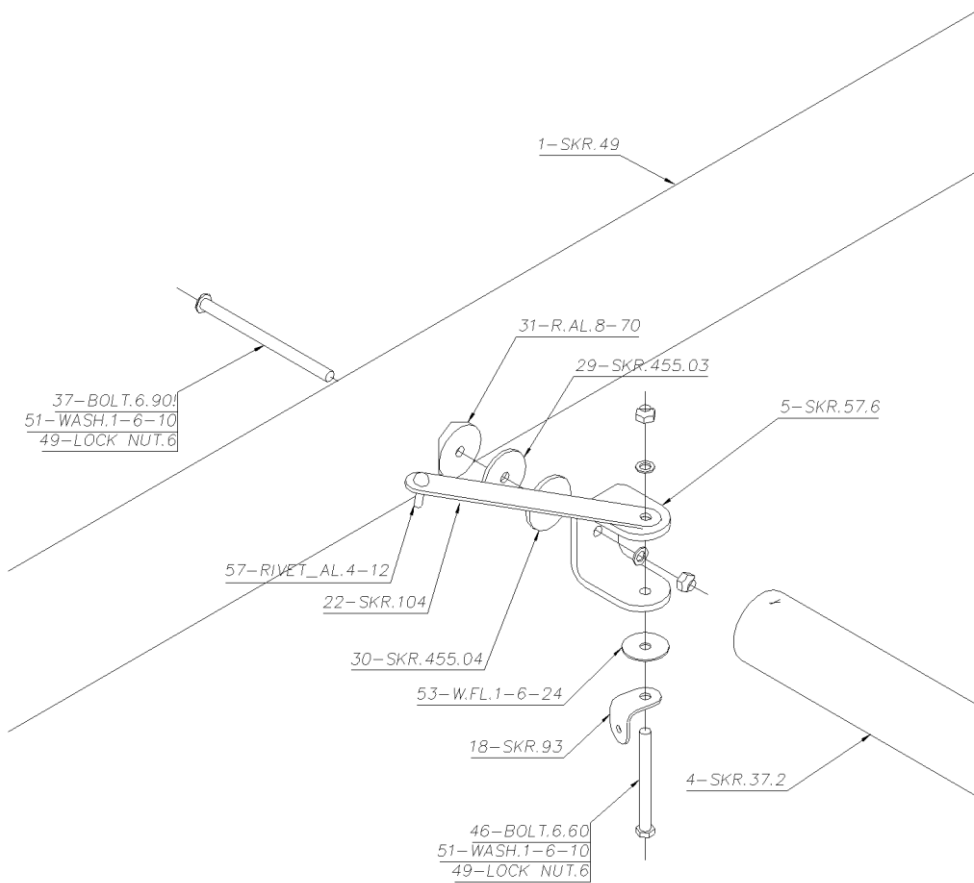
Figure 135 front jury strut attachment.
