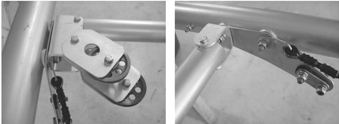
Figure 137 lift strut attachments.
