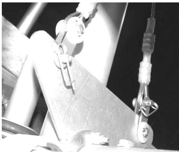
Figure 149 aileron cable connections viewed from beneath.
