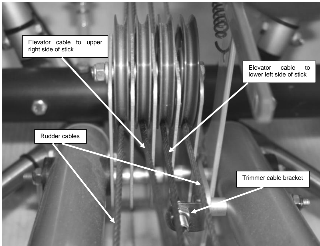
Figure 107 Nynja central pulley block arrangement loking rearwards
