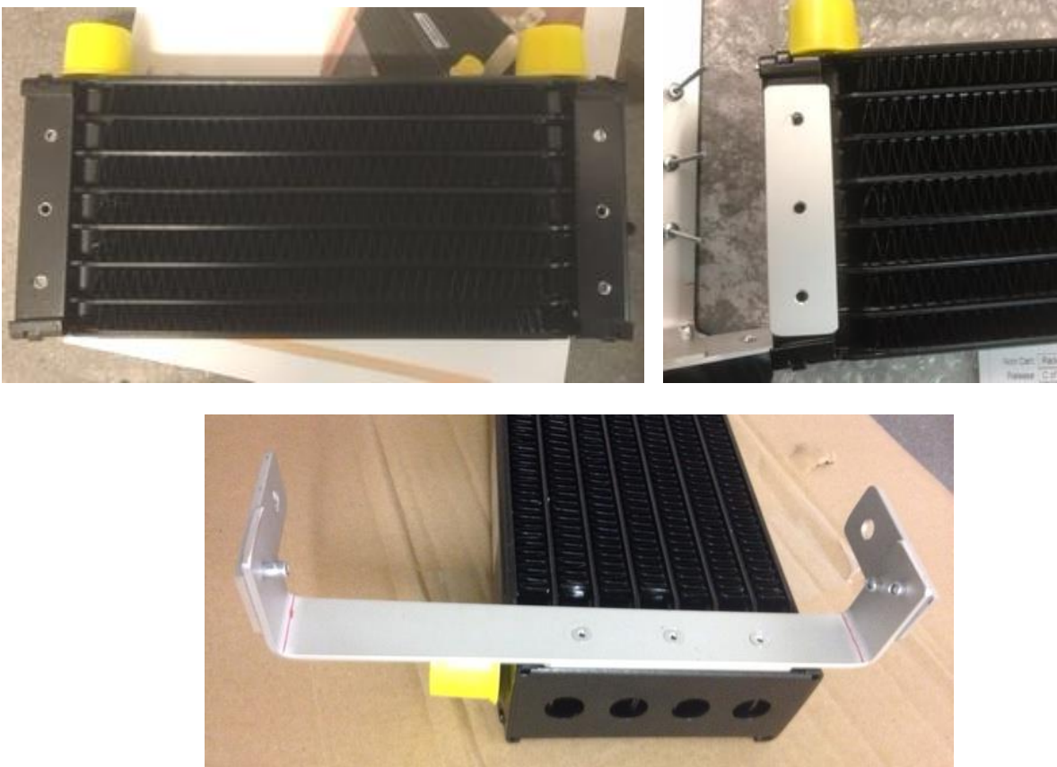
Figure 203 drilling and fixing the oil cooler to the brackets.
