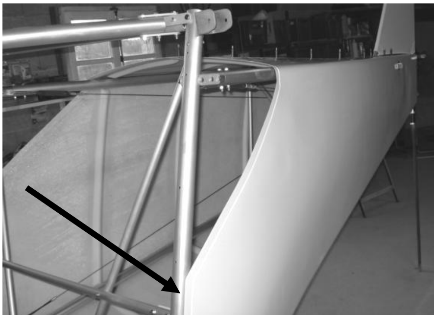
Figure 119 showing alignment of rear fairing with TU6 upright tube.
