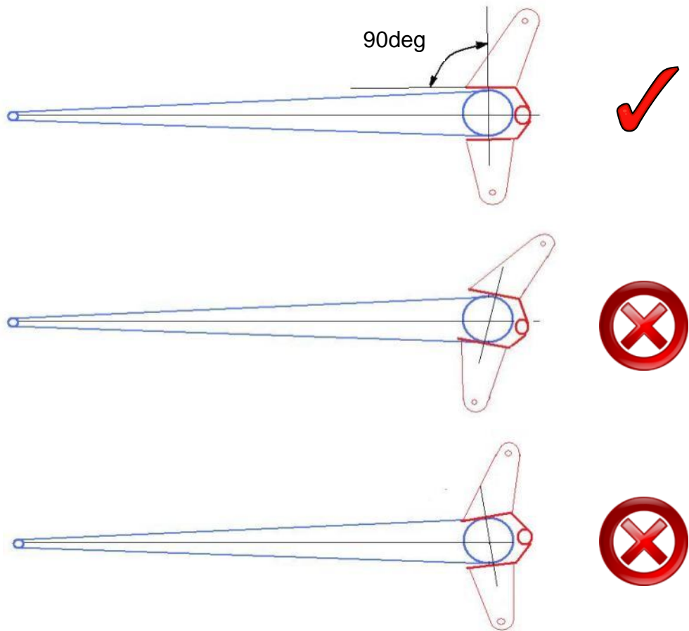
Figure 100 Nynja elevator joiner with integral control horn
