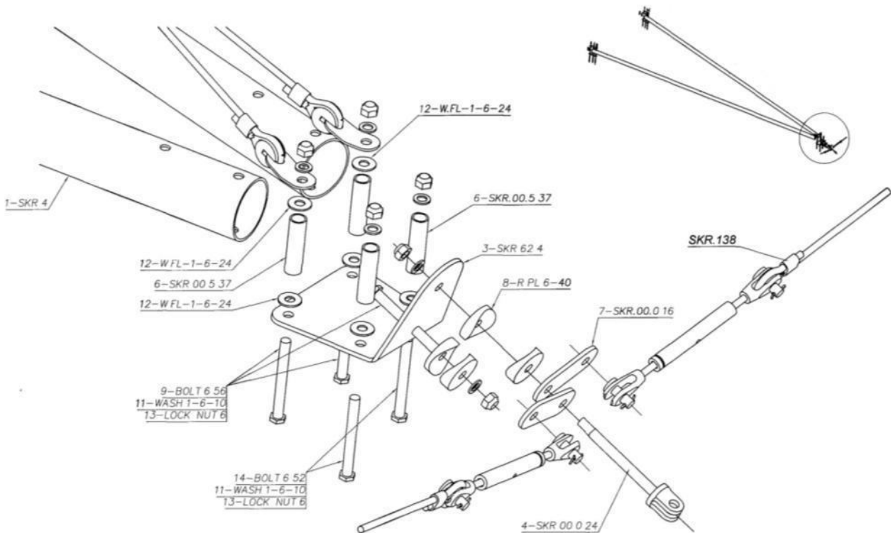
Figure 59 rear end of lower rear fuselage tubes.
