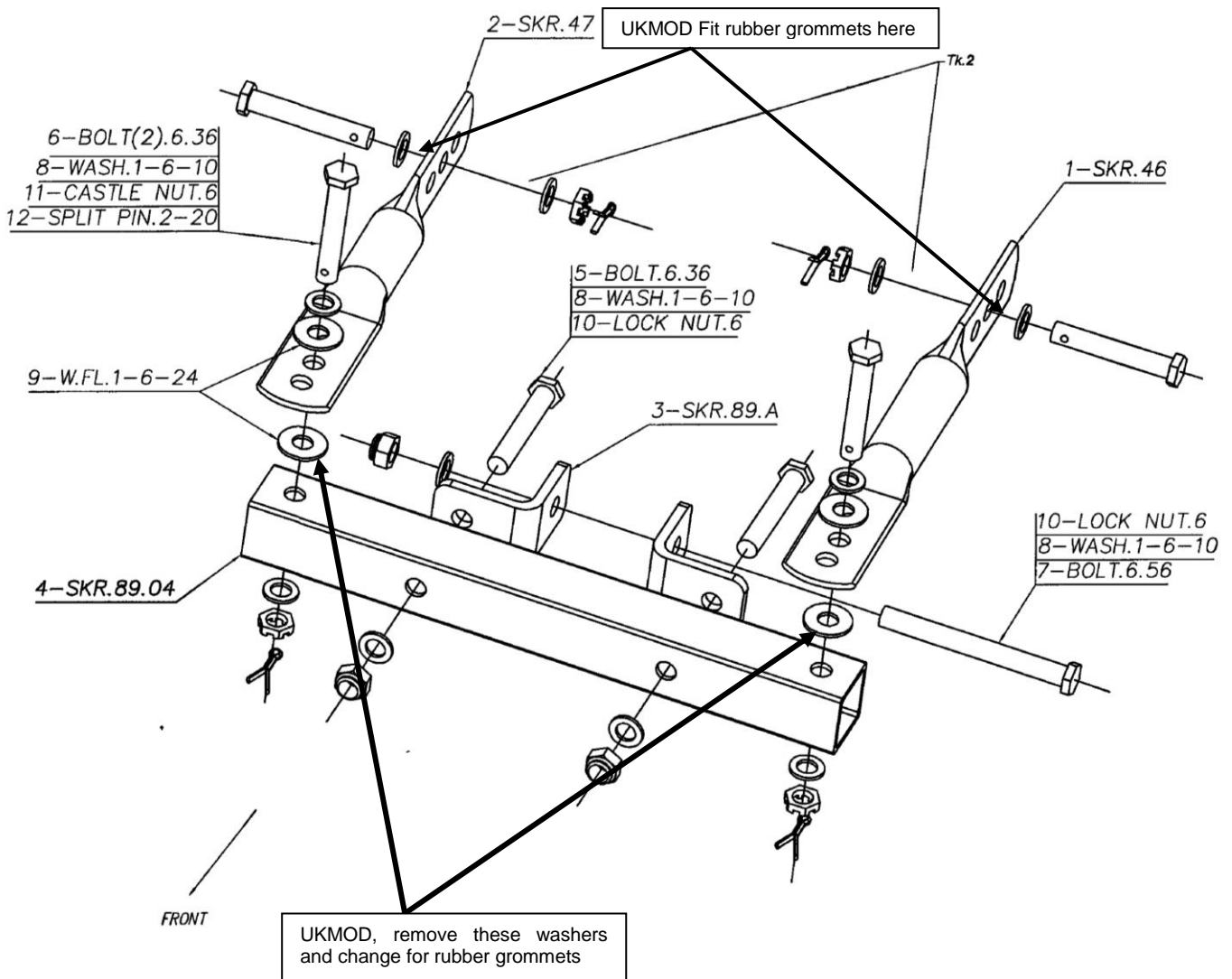
Figure 86 Nose wheel steering.
