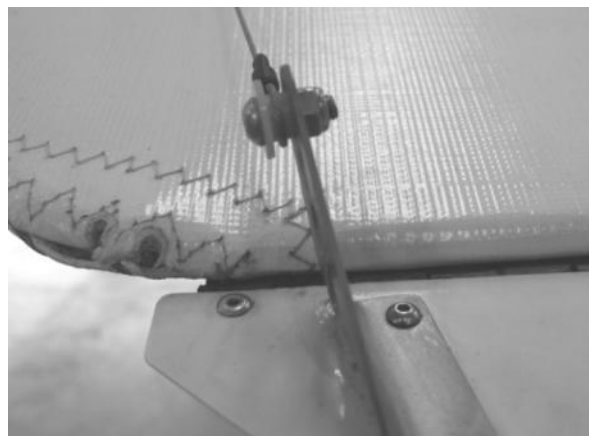
Figure 320 cable attachment on trim tab horn.
