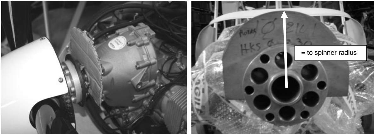
Figure 192 cowling support - horseshoe shaped to fit behind engine drive flange.
