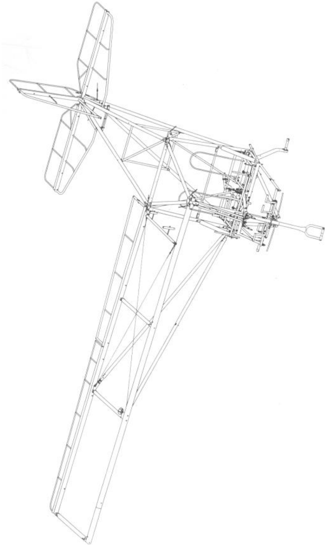
Figure 2 Basic frame (Skyraider).
