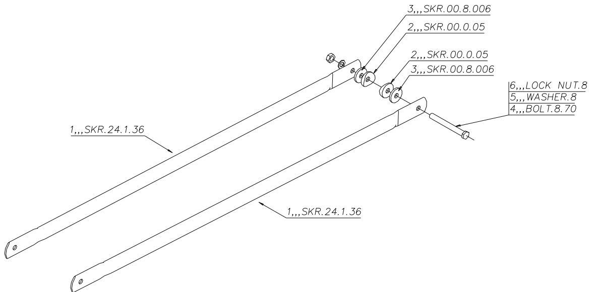
Figure 41 upper engine mount triangulation tubes.
