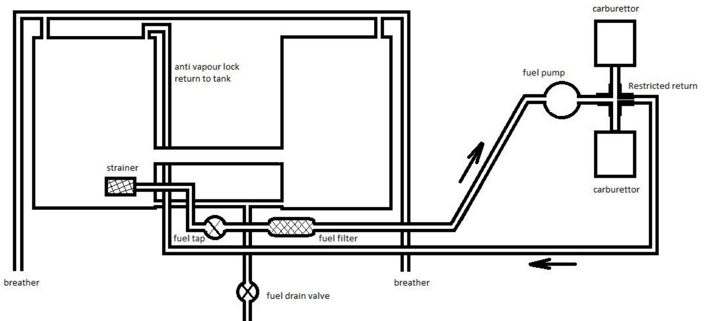
Figure 215 fuel system schematic, Rotax 912.
