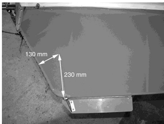
Figure 318 position of hole in top elevator surface.
