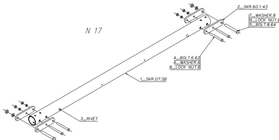
Figure 23 upper rear cabin cross-piece.
