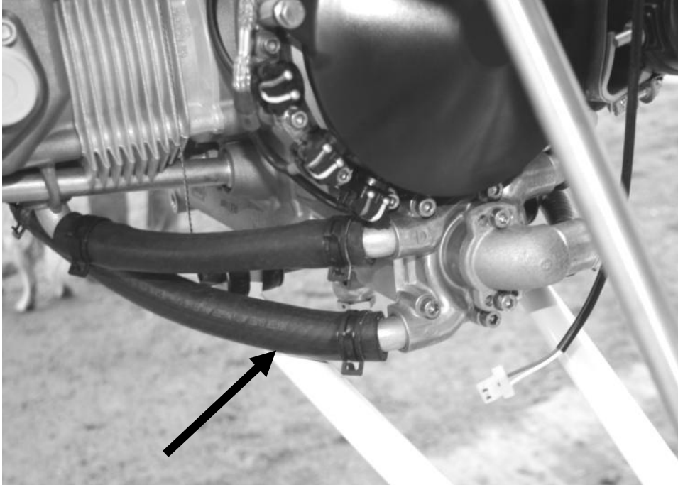
Fig 129 area of possible fouling between water pipe and lower engine mount
