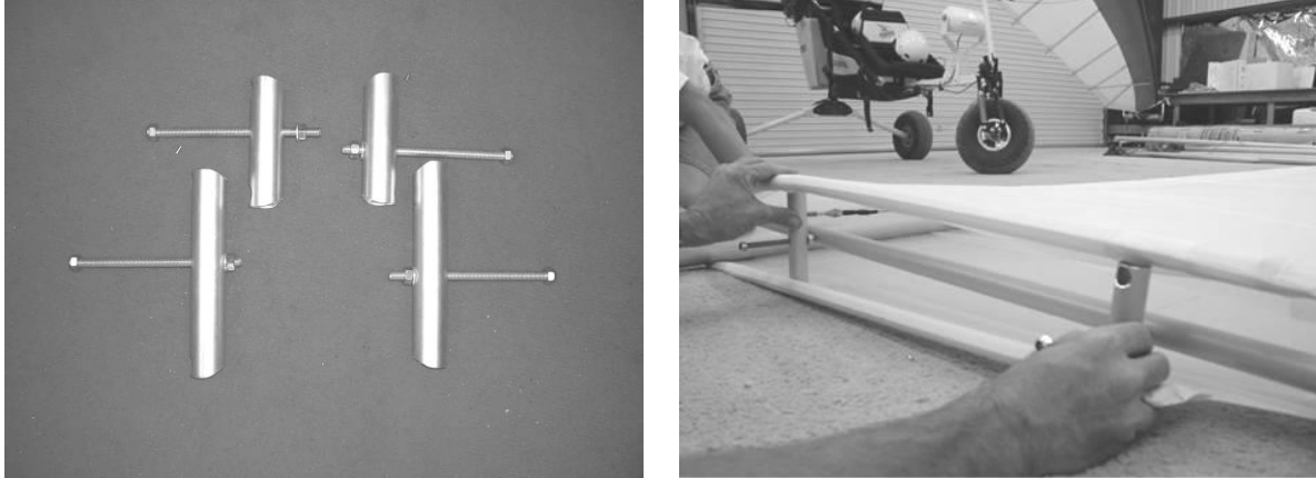
Figure 187 tensioning tubes.
