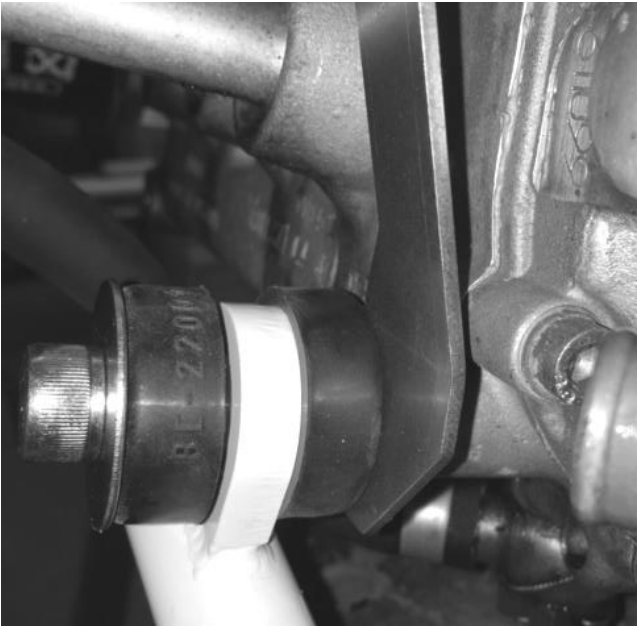
Fig 128 Overview and views of the upper and lower attachment points of the bracing strap
