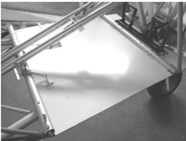
Figure 49 view of installed floor.
