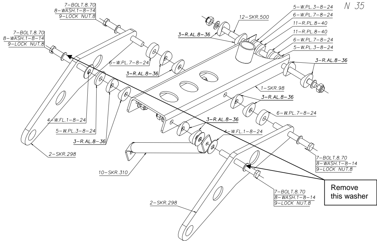
Figure34 Rotax 912 mounting bracket – note position of TU310 is reversed for Nynja – as shown correctly below
