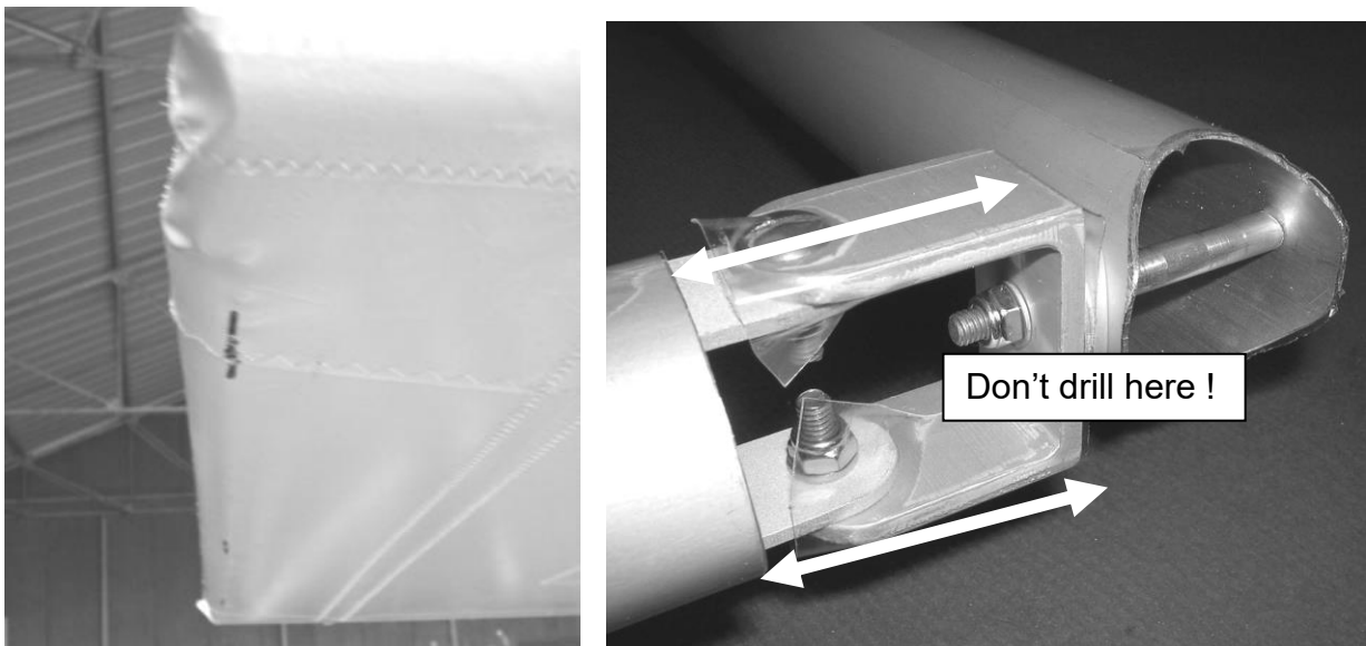
Figure 356 Wing tip
