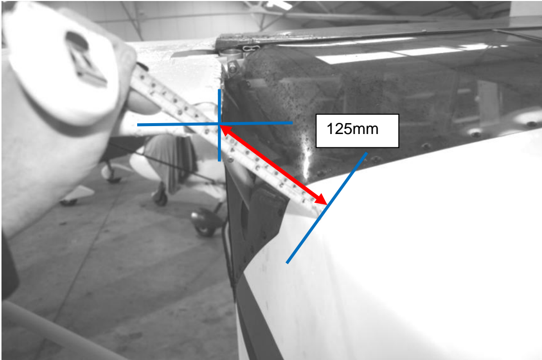
Figure 371 flap neutral setting.
