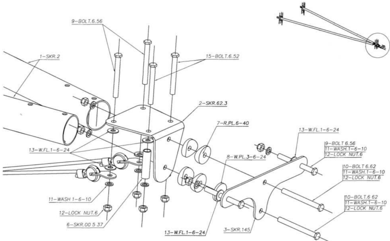
Figure 58 rear end of upper rear fuselage tubes.
