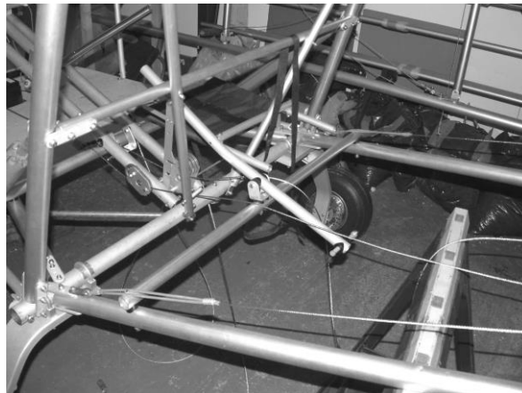
Figure 70 flap handle and fuel tank support bar.
