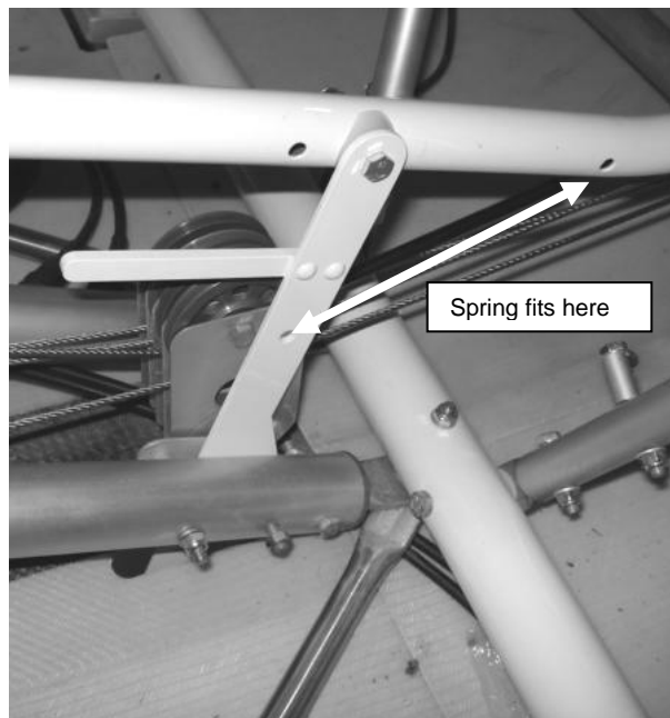
Figure 72 flap lever detail
