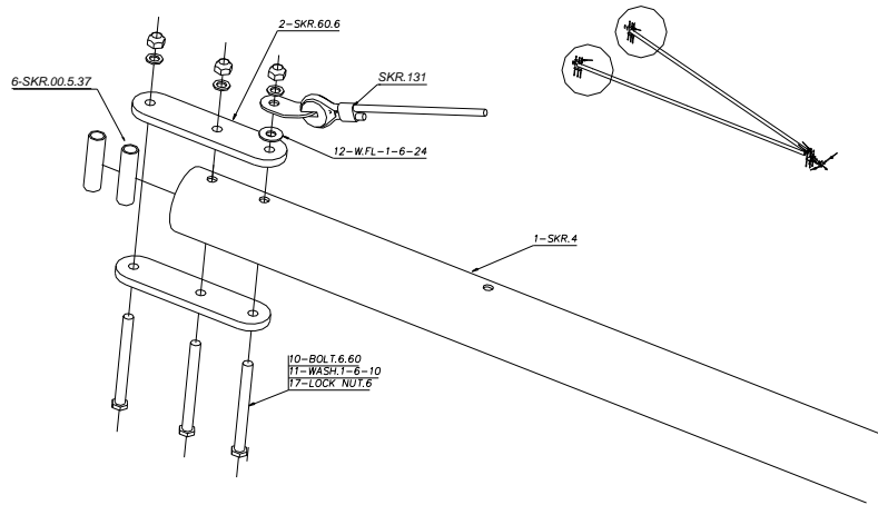
Figure 61 forward end of lower rear fuselage tubes Note upper tubes have brackets orientated at 90 degrees from that shown and cables are arranged differently on Nynja. See Figure(s) 62
