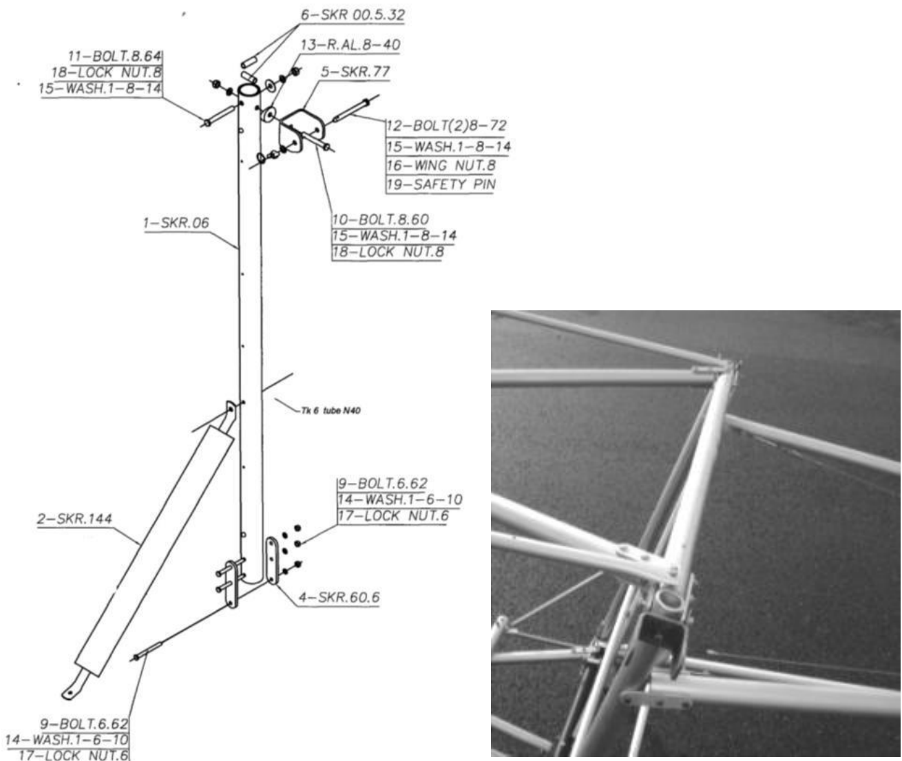
Figure 27 rear cabin uprights and correct handing for attachment of SKR2 fuselage longerons
