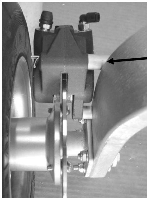
Figure 89 spacers on brake mounts.
