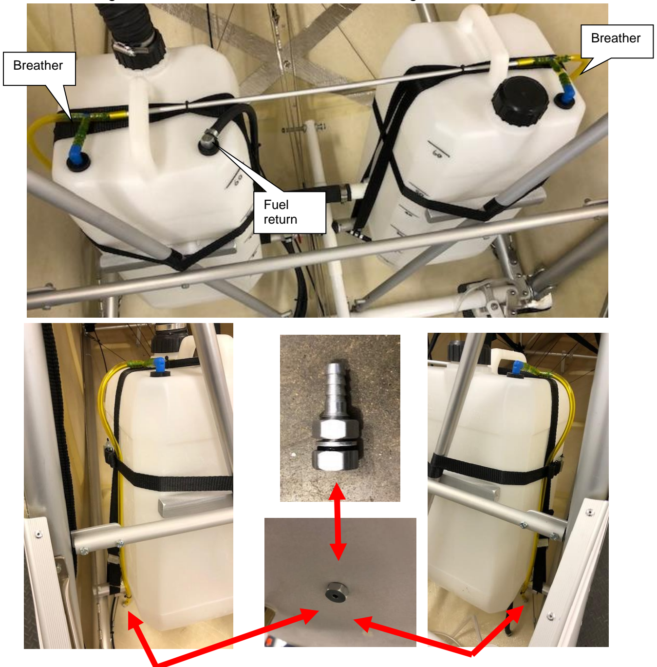
Figure 231 fuel tank breathers
