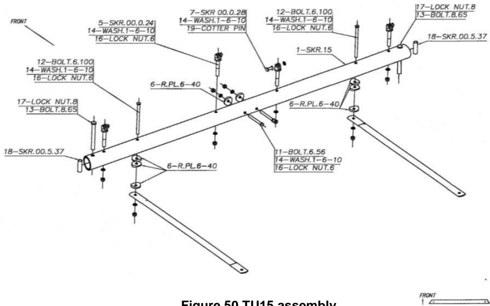
Figure 50 TU15 assembly
