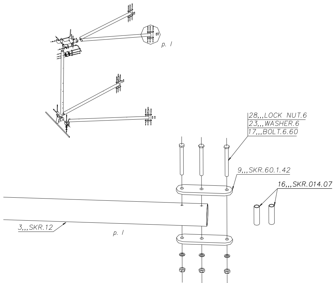
Figure 24 rear of upper cabin triangle tube tu10.
