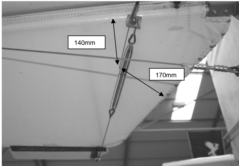
Figure 319 position of hole in lower elevator surface.
