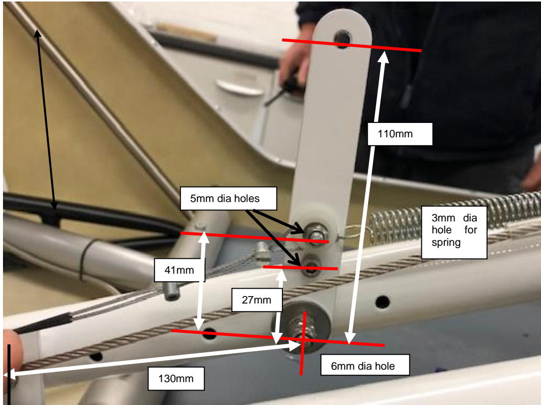
Figure 321 trim lever
