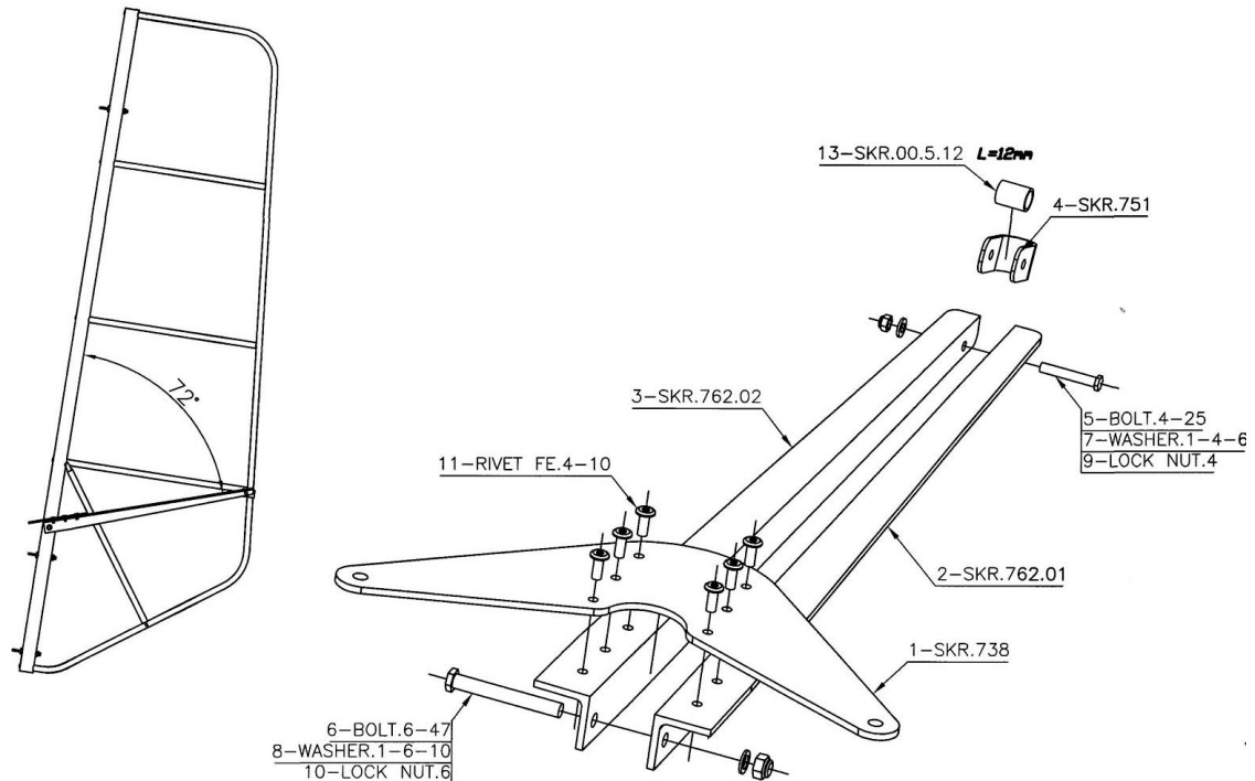
Figure 101 rudder horn assembly (note: Skyranger rudder frame shown. Nynja Rudder is slightly different shape).
