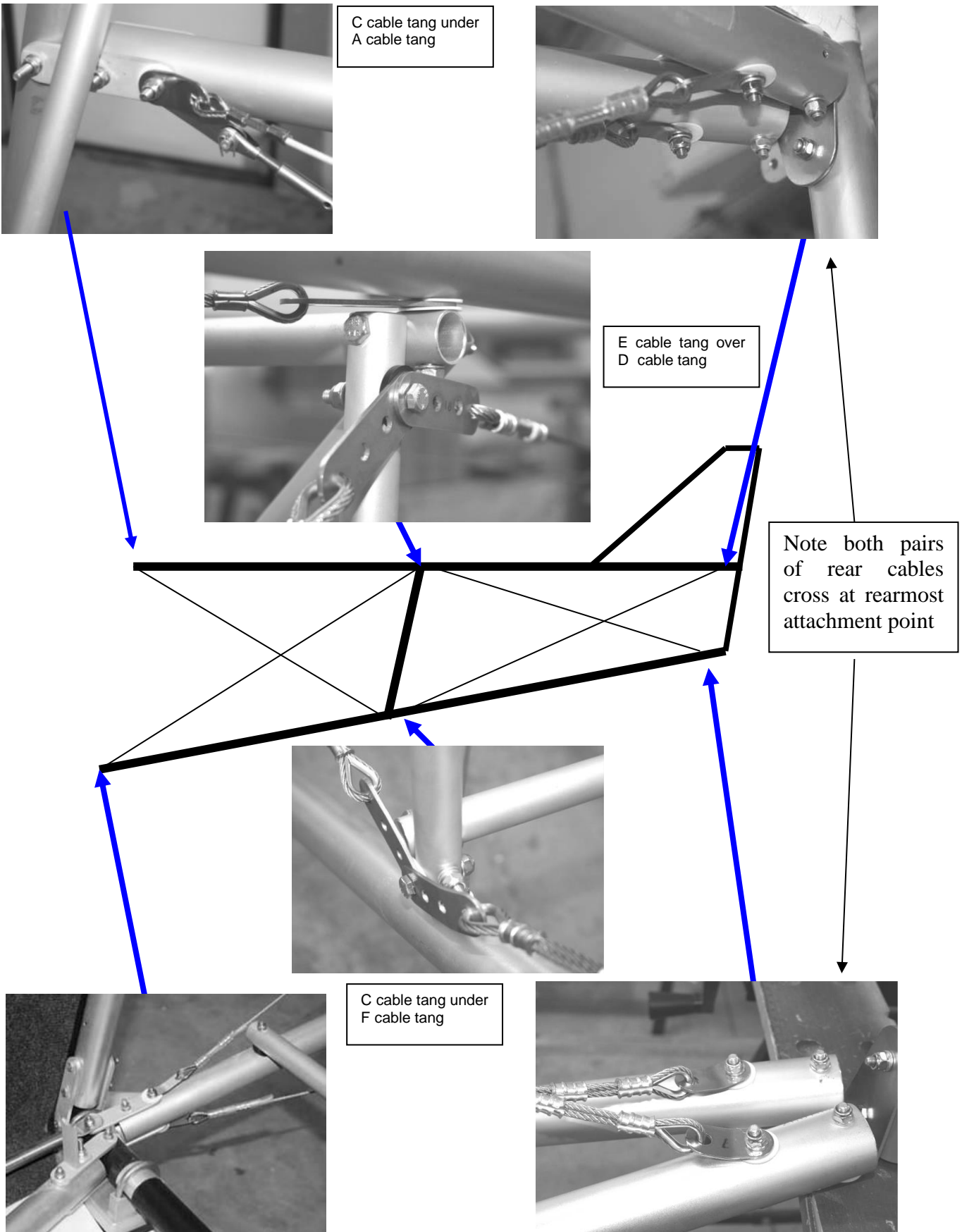
Figure 64 fuselage cable ends detail
