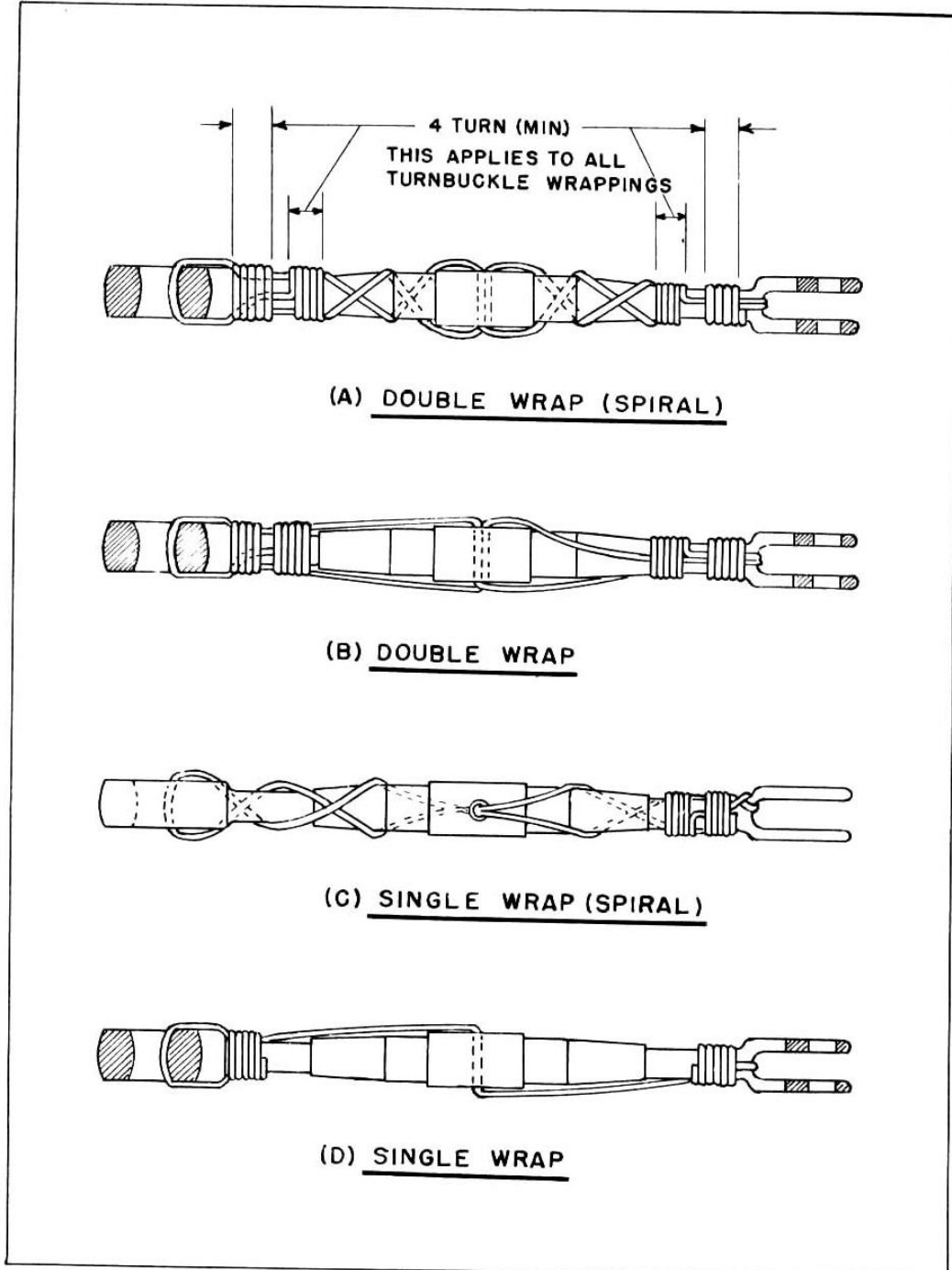
FIGURE 4.23.—Safetying turnbuckles.
