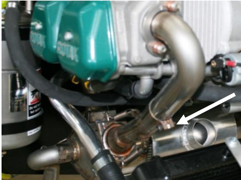
Figure 199 Port front pipe, showing clamp on sliding section
