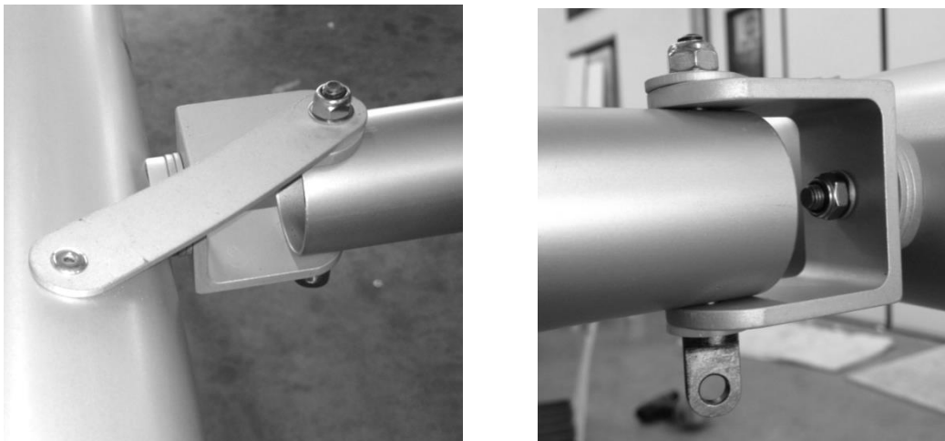
Figure 134 forward and rearjury strut attachments.
