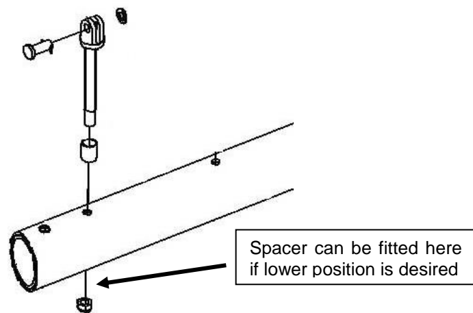
Figure 335 Front fixing
