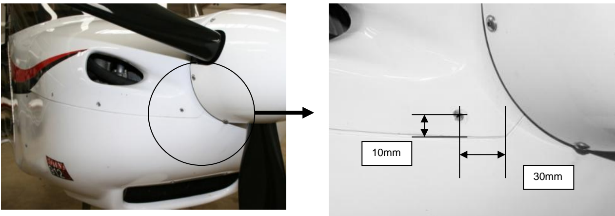
Figure 189 front cowling fixing
