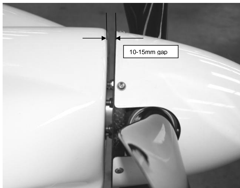
Figure 193 spinner / cowling alignment
