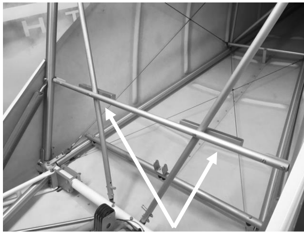
Figure 32 fuel tank wooden tank spreader pieces.
