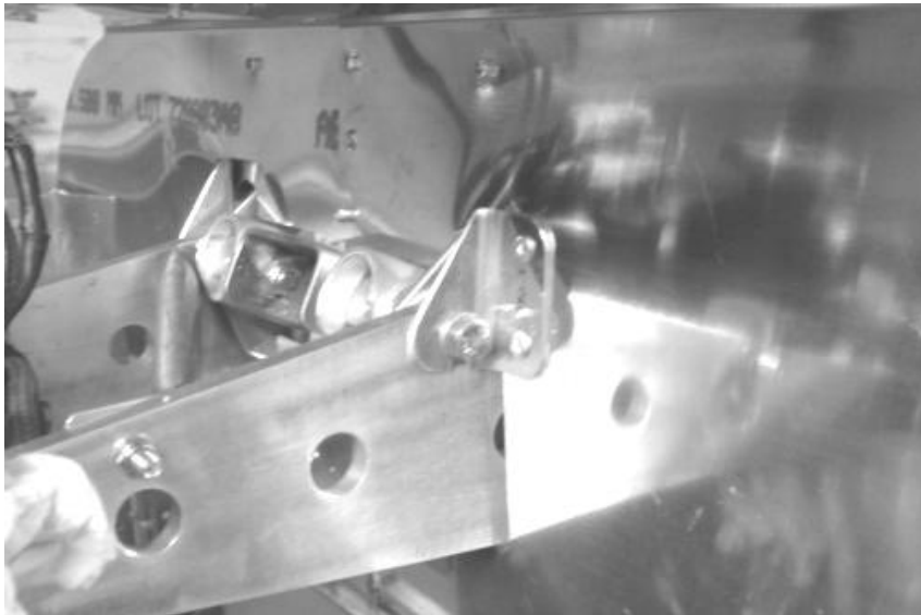
Fig 36 Nynja firewall support brackets, should be fitted on the engine mount bolts at the front of the SKR19's at this stage as shown (normally found packaged with the instrument panel angles)
