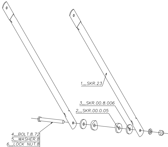
Figure 42 lower engine mount triangulation tubes.
