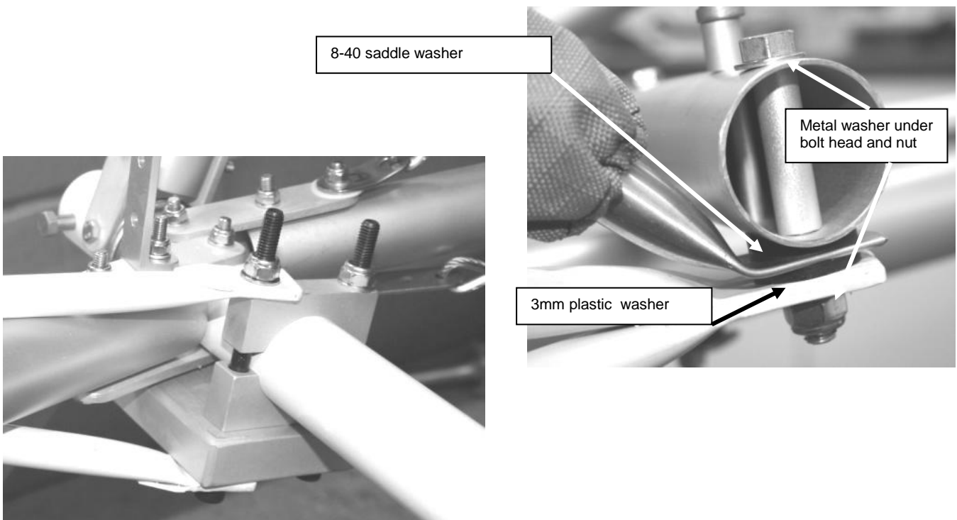
Figure 83 rear and forward ends of starboard drag brace
