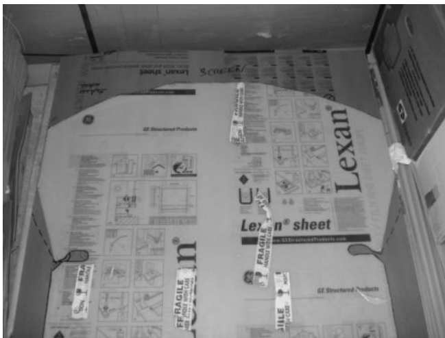
Figure 287 cutting the Lexan to the pattern.
