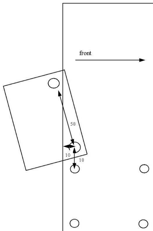
Figure 78 hole for brake calliper mounting.
