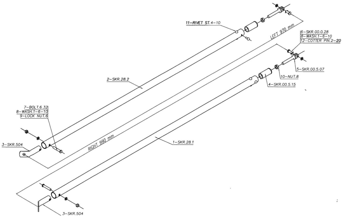
Figure 153 flap handle, looking rearwards and flap rods (note Nynja flap rods have slight bend in upper ends, not shown in this drawing)
