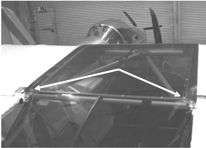
Figure 288 drilling for the rear mounting bolts.
